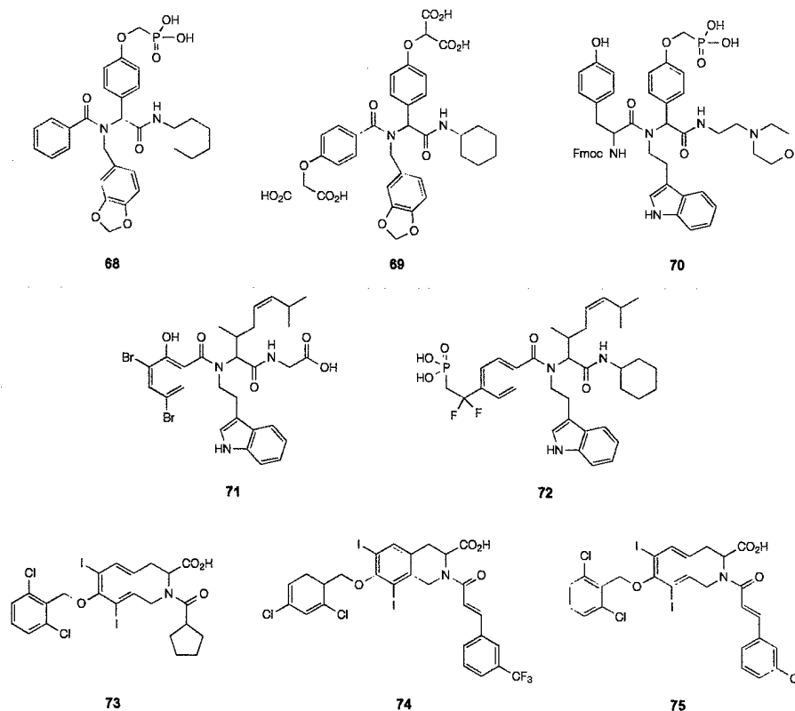
Figure 9 | Synthetic inhibitors.
