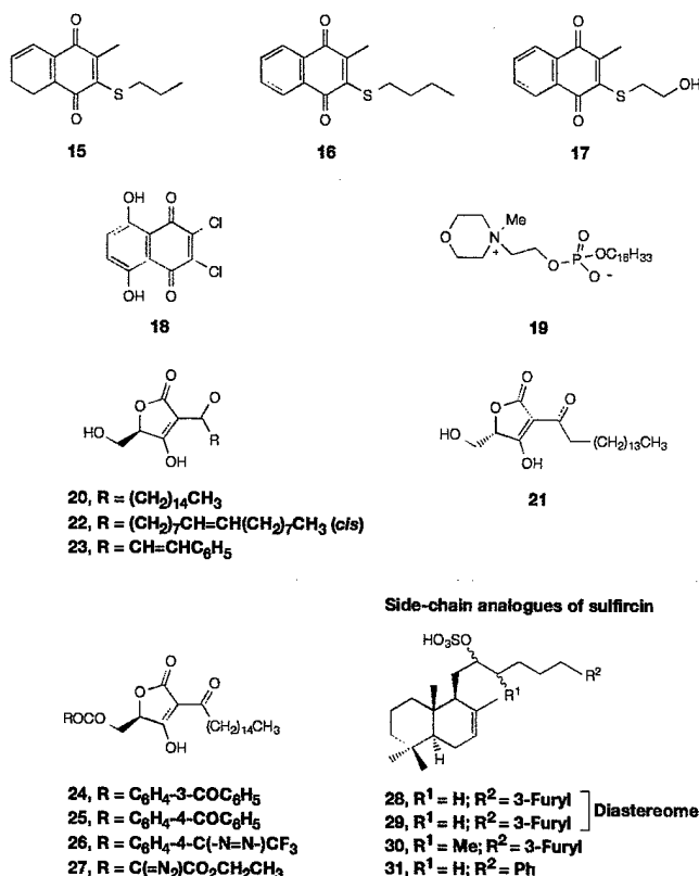
Figure 5 | Natural-product analogues. Me, methyl group; Ph, phenyl group.
