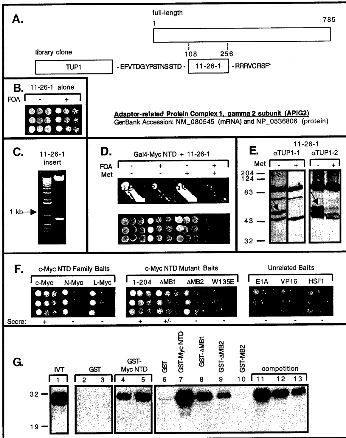
Figure B18. Library clone 11-26-1, Adaptor-related Protein Complex 1, gamma 2 subunit (APIG2) (A) Schematic representation of the TUP1-fusion library clone against the full-length protein sequence (B) Expression of the library clone alone on +/-FOA (C) EcoRI/BamHI restriction digest to release cDNA insert from pBDH vector (D) Original selection on +/-FOA, +/-Met (upper panel); Retransformation of library clone with Gal4-Myc NTD bait into fresh yeast cells on +/-FOA, +/-Met media (lower panel) (E) \alpha Tup1 immunoblot analysis of Tup1-fusion expression under +/-Met conditions, specific bands marked by an arrow (F) Coexpression of library proteins with Myc-related and -unrelated activator baits on +FOA, score is relative to growth with c-Myc (G) In vitro translation (IVT) of library protein, binding experiments using crude lysates of recombinant GST-fusion proteins (lanes 2-10) and competition experiments using purified GST-free Myc NTD (lanes 11-13).
