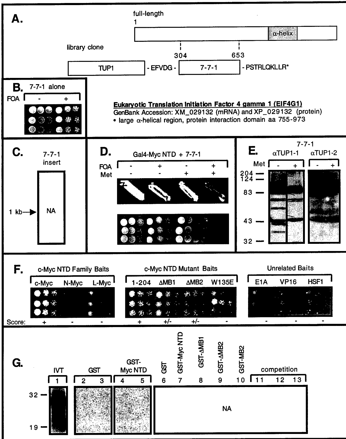
Figure B8. Library clone 7-7-1, Eukaryotic Translation Initiation Factor 4 gamma 1 (EIF4G1)
