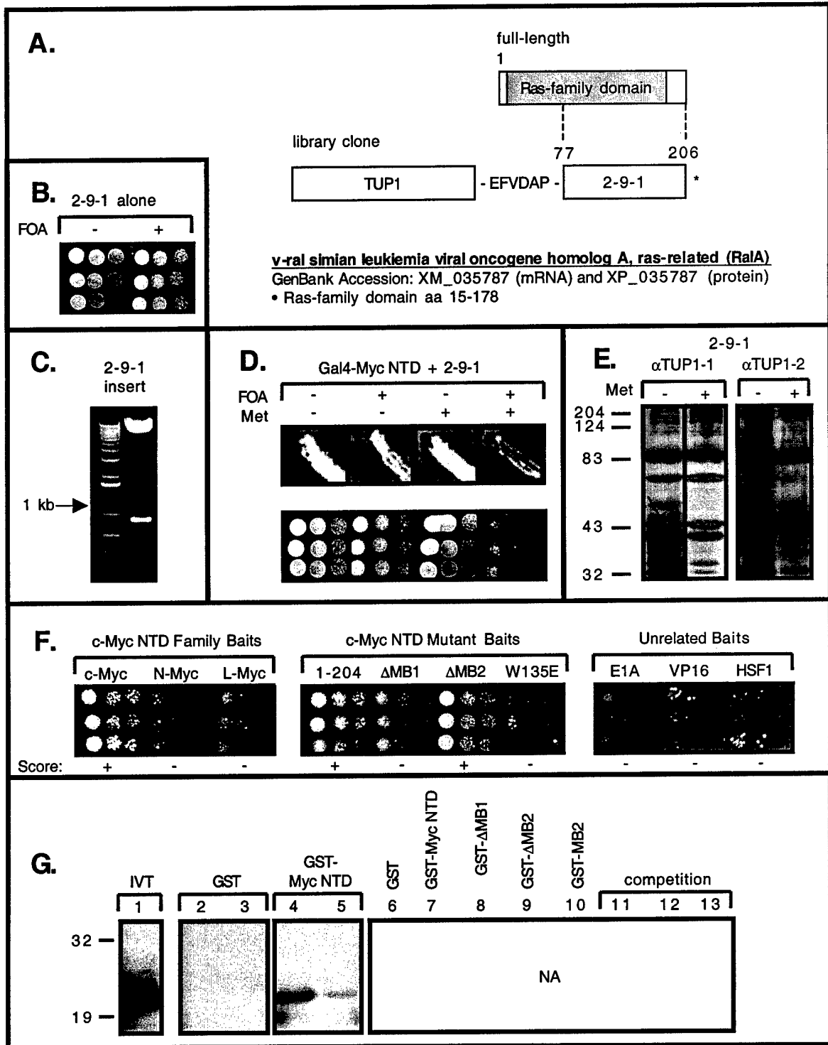
Figure B3. Library clone 2-9-1, v-ral simian leukemia viral oncogene homolog A, ras-related (RalA) (A) Schematic representation of the TUP1-fusion library clone against the full-length protein sequence (B) Expression of the library clone alone on +/-FOA (C) EcoRI/BamHI restriction digest to release cDNA insert from pBDH vector (D) Original selection on +/-FOA, +/-Met (upper panel); Retransformation of library clone with Gal4-Myc NTD bait into fresh yeast cells on +/-FOA, +/-Met media (lower panel) (E) αTup1 immunoblot analysis of Tup1-fusion expression under +/-Met conditions, specific bands marked by an arrow (F) Coexpression of library proteins with Myc-related and -unrelated activator baits on +FOA, score is relative to growth with c-Myc (G) In vitro translation (IVT) of library protein, binding experiments using crude lysates of recombinant GST-fusion proteins (lanes 2-10) and competition experiments using purified GST-free Myc NTD (lanes 11-13).
