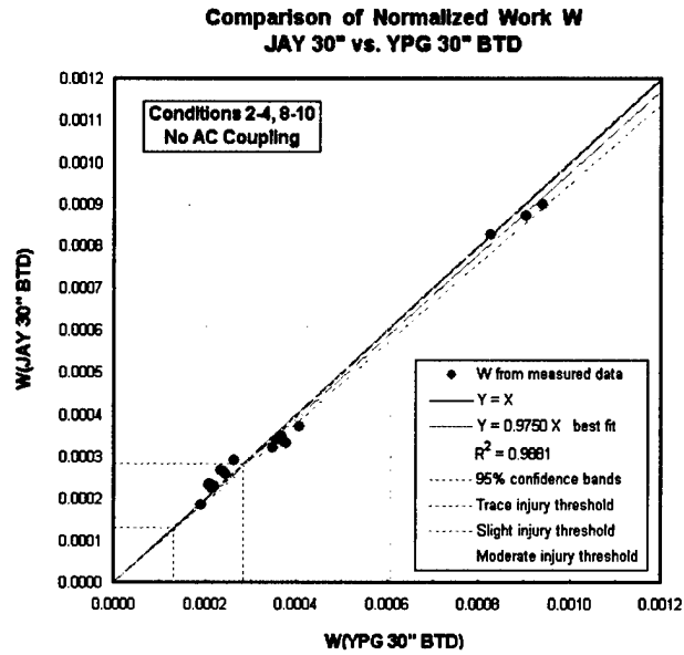
Scatter plot and linear regression comparing W for the Jaycor 30" BTB and YPG 30" BTBs.
