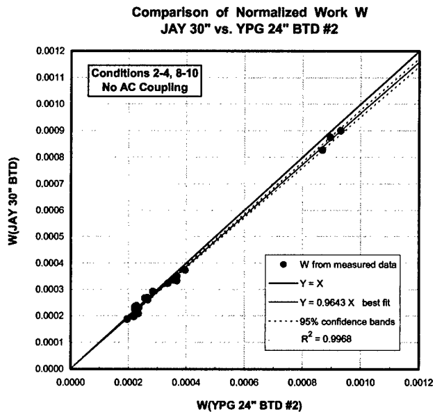
Scatter plot and linear regression comparing W for the Jaycor 30" BTB and YPG 24" BTB #2.
