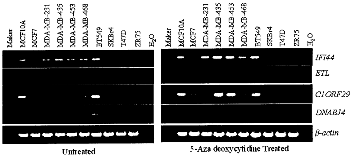
Figure 4. Effect of 5-Aza-2'-dC treatment on the restoration of gene expression. Expression of candidate genes from the 1p31 reitical region 10 breast cancer cell lines before and after treatment with the demethylating agent 5-Aza-2'-dC (10 μM) for 10 days. For the four genes shown in this figure, gene expression was restored in at least one cell line after treatment of cells in culture with the demethylating agent 5-Aza-2'-dC. Gene expression was detected by RT-PCR from total RNA extracted from treated or untreated cells. Amplification of β-actin was used to normalize the cDNA concentration.
