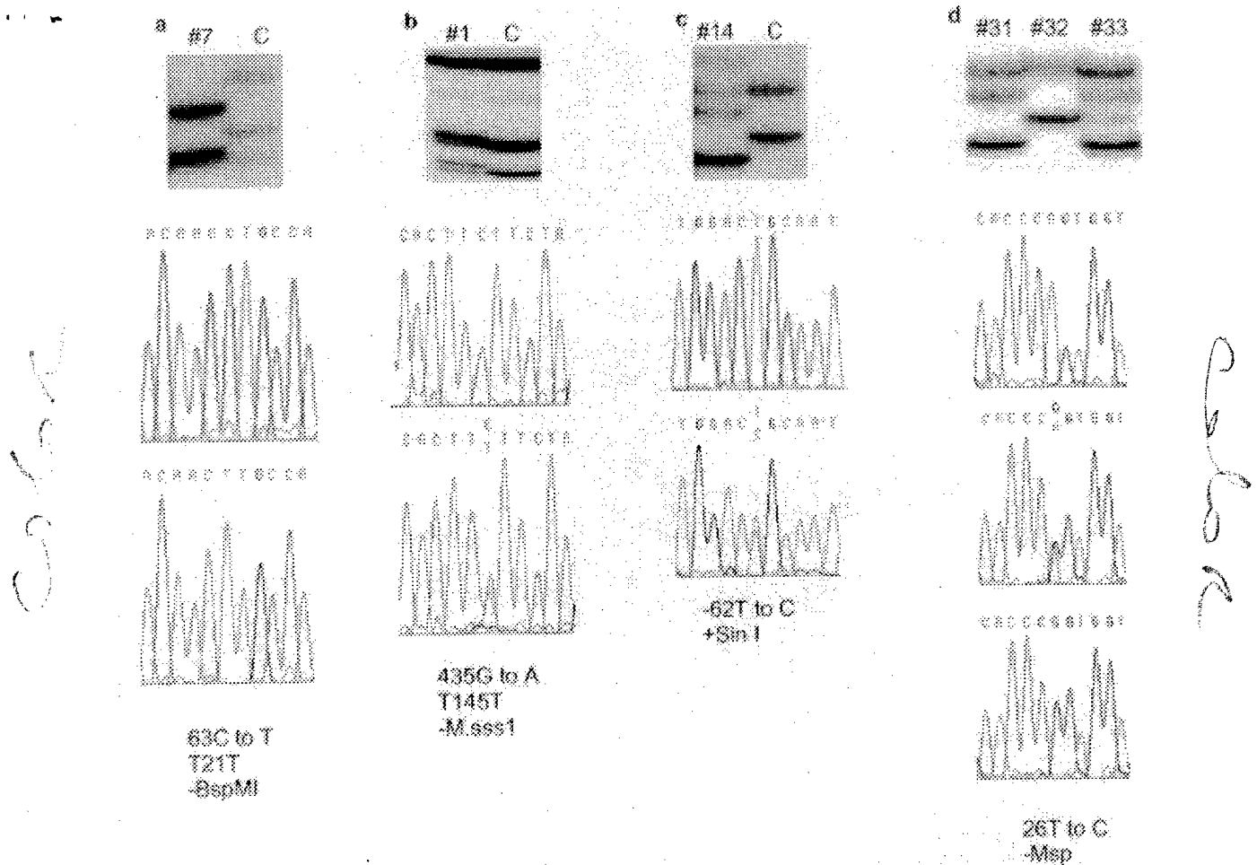
Figure 2. Detection of single nucleotide variations using IPS. Four different SSCP shifts were detected in different breast cancer tumors and are shown in the upper panels of a-d, respectively. Nucleotide sequences corresponding to each SSCP change are shown in the lower panels of a-d, respectively. The nucleotide variation, amino acid change and restriction enzyme site alteration are listed below the sequence traces.
