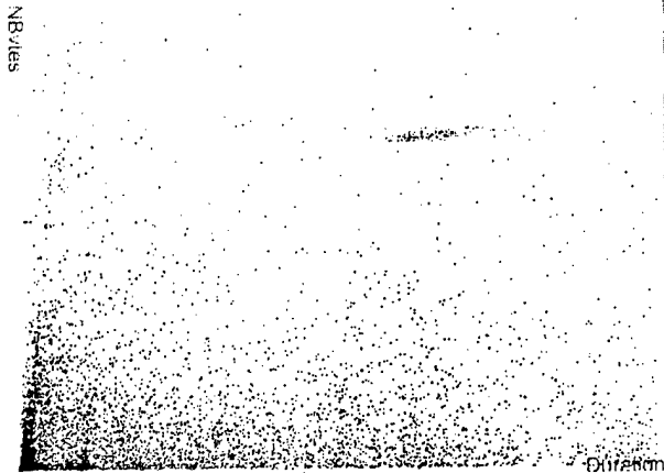
Figures 6a and 6b: Anomaly detected and highlighted in red in drilled down plot of the Number of Bytes versus Duration. The same data are shown in 6b in a parallel coordinate display indicating that the anomalous packets shared the same destination IP, port, and source IP.
