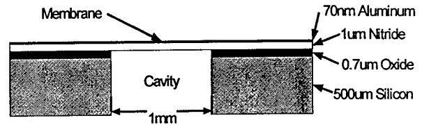
Figure 2. Cross section of MEMS diaphragm.
