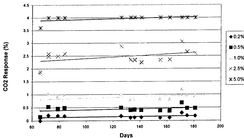
Figure 17. Draeger CO2 Performance
