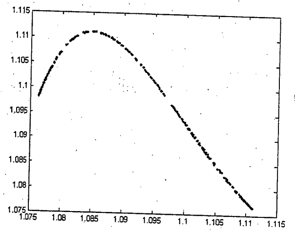
Fig. 30. Reconstructed phase portrait, Poincare section (left) and quasi-one-dimensional map for \varepsilon = 0.446 for different Poincare cross-sections.
