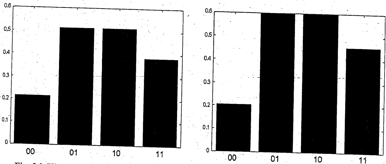
Fig. 36. Histograms of relative frequencies of permitted sequences of length 2 for two different methods of construction of binary sequence of the system (8).
