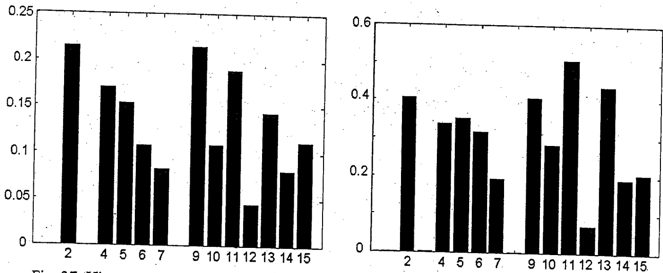
Fig. 37. Histograms of relative frequencies of permitted sequences of length 4 for two different methods of construction of binary sequence of the system (8).
