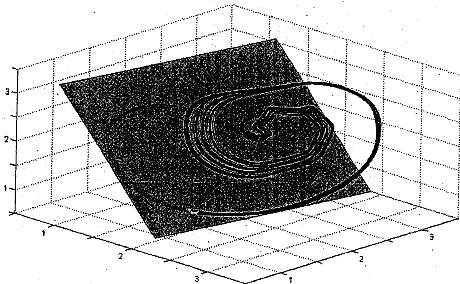
Fig. 32. Trajectory in reconstructed phase space and Poincaré section for \varepsilon = 0.443
