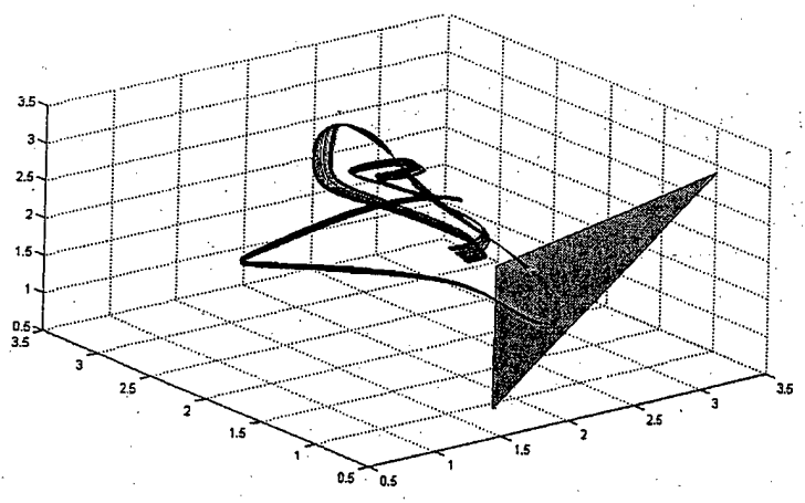
Fig. 30. Reconstructed phase portrait, Poincare section (left) and quasi-one-dimensional map for \varepsilon = 0.446 for different Poincare cross-sections.
