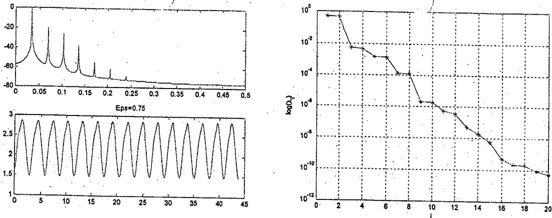
Fig. 11. Power spectrum, waveform and spectrum of eigenvalues of covariance matrix for system (8) at \alpha = 2.05 , \beta = 1.45 , \epsilon = 0.75 .
