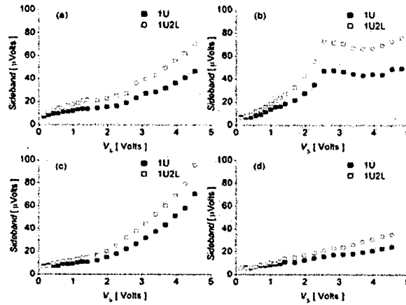
FIG. 5. Comparison between one-carrier and two-carrier operation of the UDV on a sand surface excited by an AURA shaker at 150 Hz. (a), (b) shaker buried ~3 cm below the surface, (c) shaker surface flush with sand surface, (d) shaker on lead bricks. V_S is the shaker excitation voltage.
