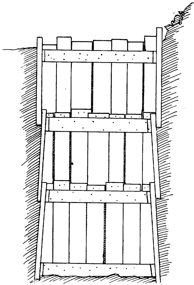
FIGURE 26.—Shaft—cross section.
