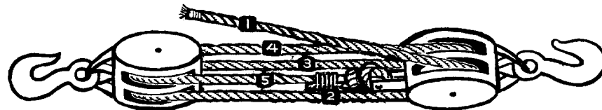
FIGURE 3.—Reeving—double and double.
