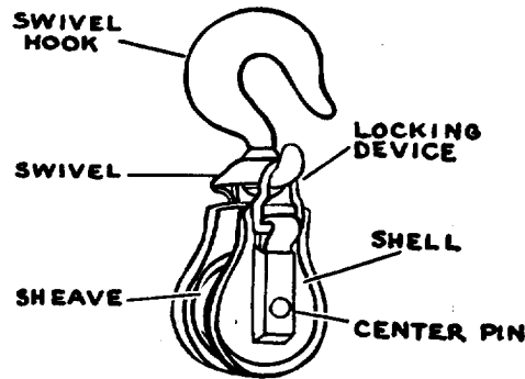
FIGURE 2.—Snatch block.
