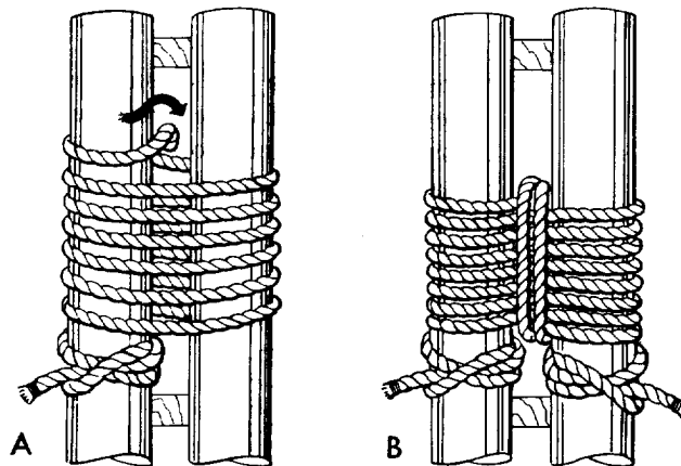
FIGURE 11.—Sheerlegs lashing.
