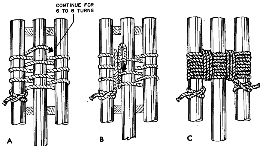
FIGURE 13.—Lashing for tripod.
