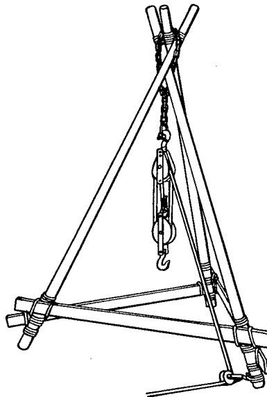
FIGURE 12.—Tripod.
