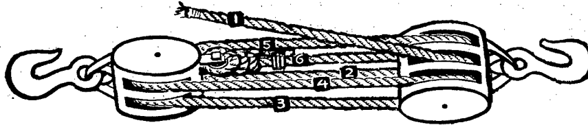
FIGURE 4.—Reeveing—triple and double.
