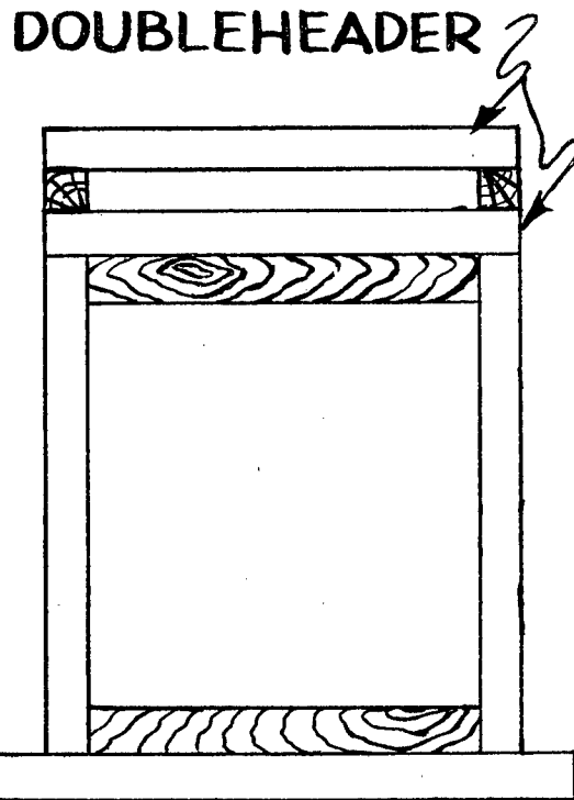
FIGURE 23.—Doubleheader (permanent).
