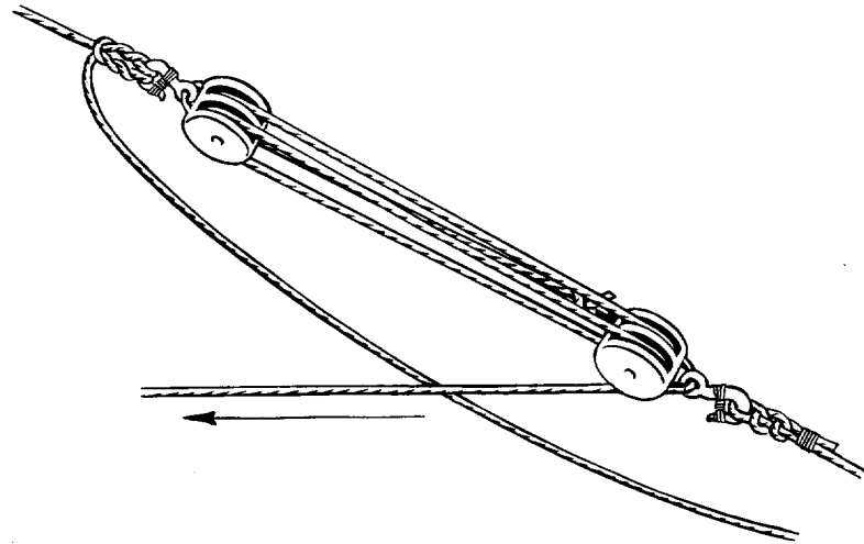
Details of luffing tackle.
