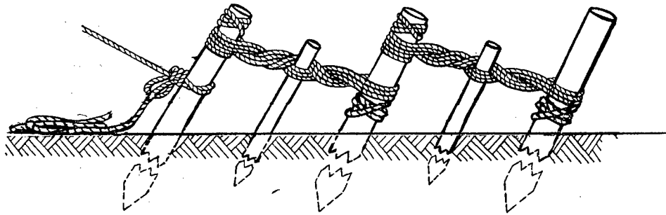
FIGURE 9.—Pickets
