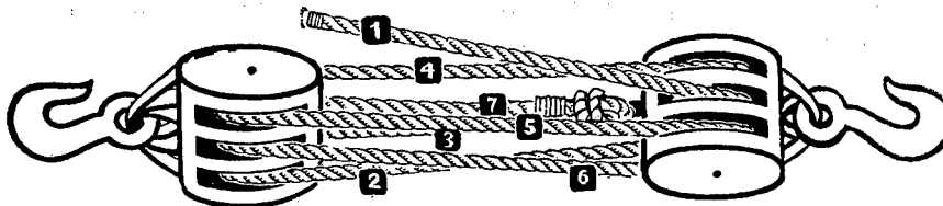
FIGURE 5.—Reeveing—triple and triple.
