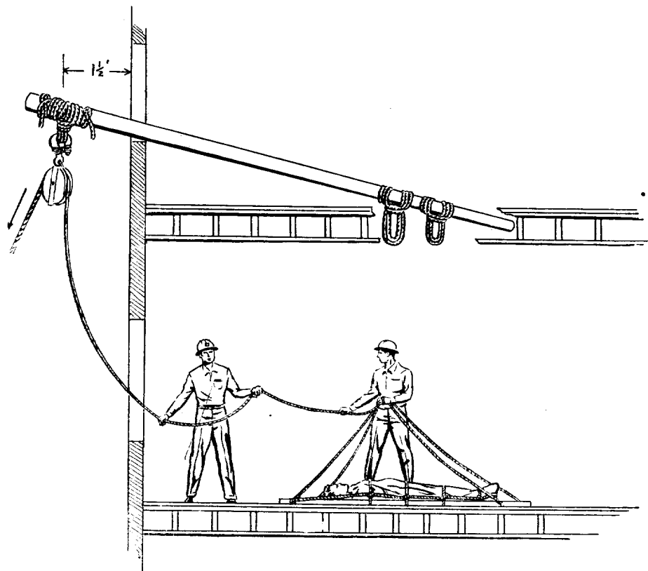
FIGURE 16.—Jib arm
