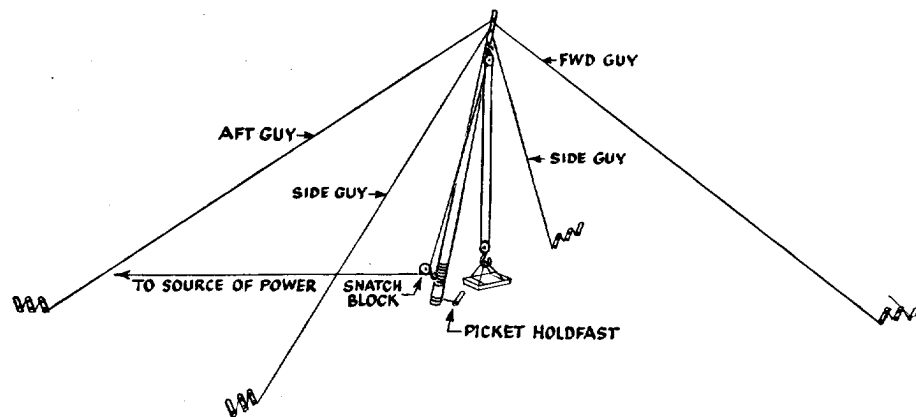
FIGURE 7.— Gin pole.
