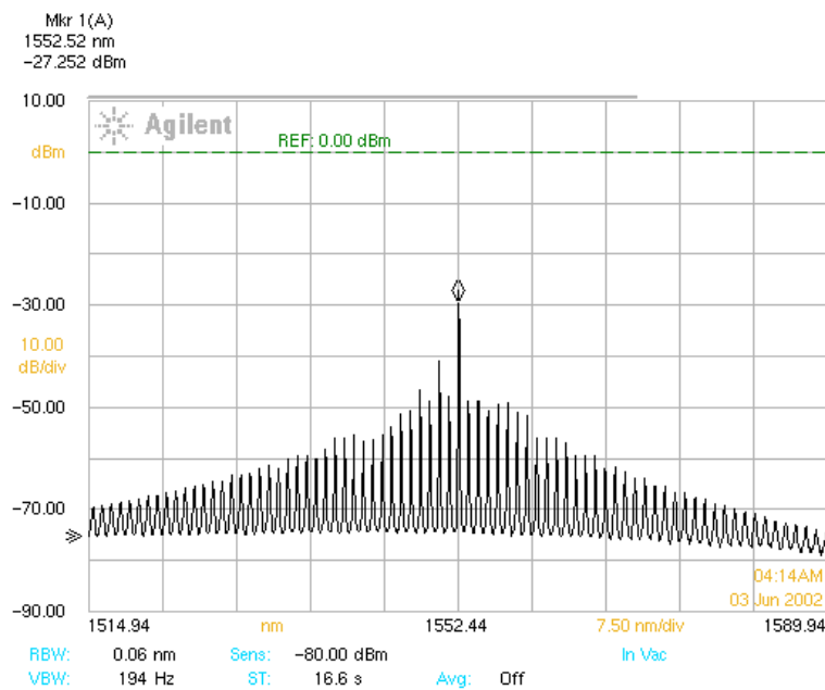
Figure 2. Spectrum of ring laser.
