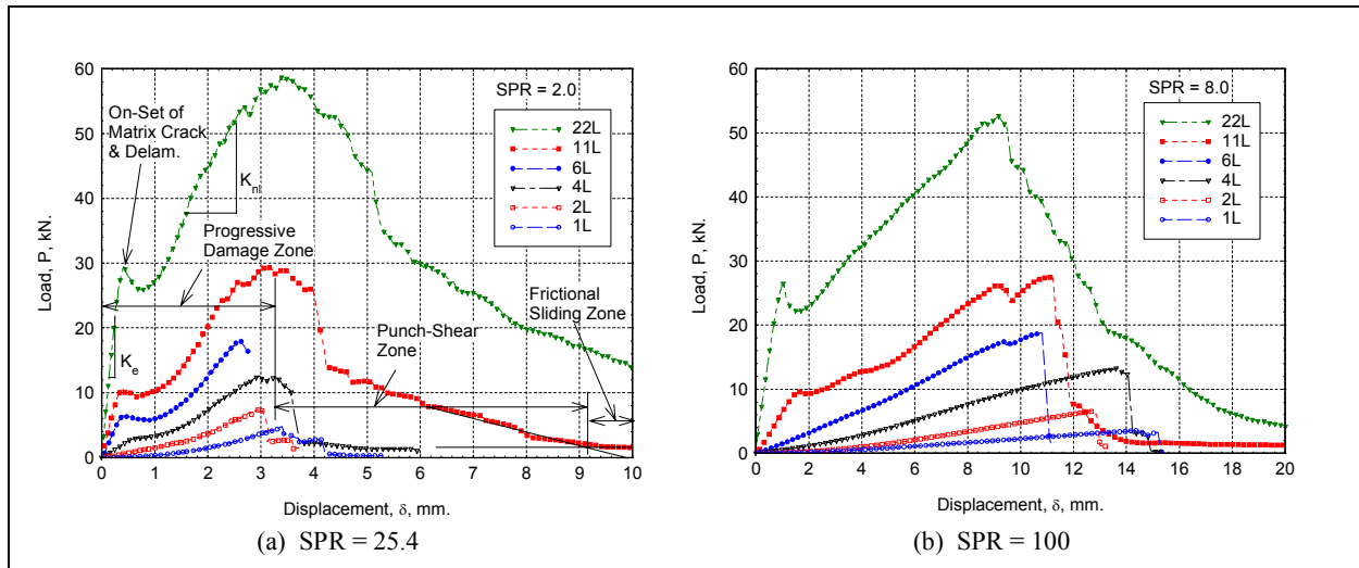
Figure 2. Punch shear behavior of 2-D baseline S-2 Glass/SC15 Composite laminates.
