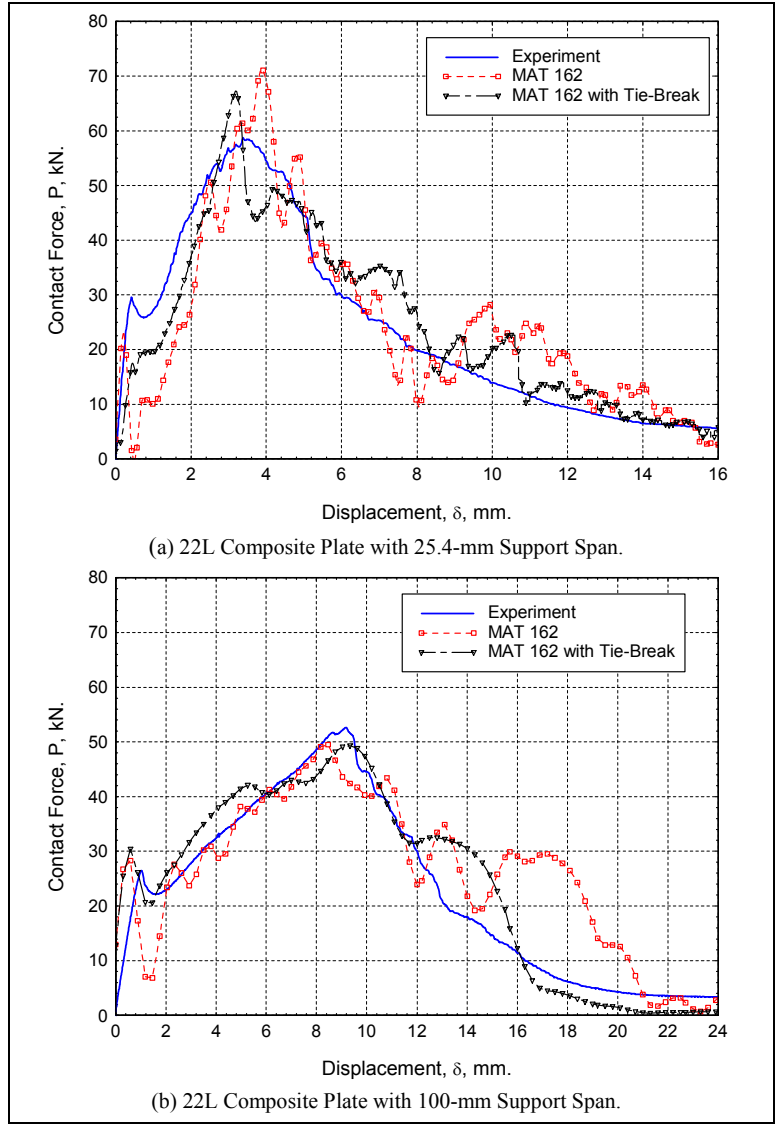
Figure 3. Comparison of contact force-displacement curves.
