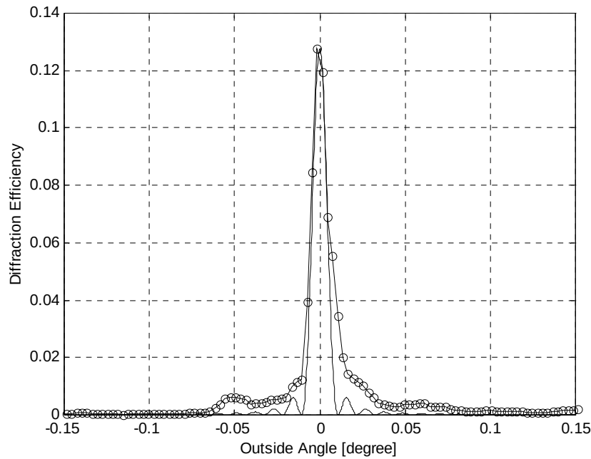
Fig. 3-5. Experimental angular selectivity curve (dots) of a hologram recorded on 5 mm thick LiNbO 3 crystal compared to the theory (solid line).
