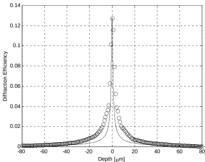
Fig. 3-4. Depth selectivity measurement (dots) of a hologram recorded on 5 mm thick LiNbO 3 crystal compared to the theoretical prediction (solid line).
