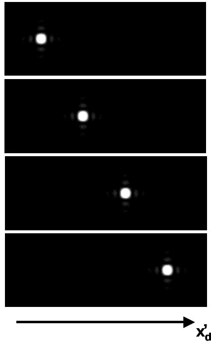
Fig. 3-14. Simulation of the intensity profile and position of the diffracted spot on the detector plane as a monochromatic point source is shifted along the x -axis in 4.5 \times \lambda steps. Simulation parameters: \lambda=514 nm, L_z=200 \mu\text{m} , f_{m0}=4.5 mm, f_i=4.5 mm and \text{NA}=0.65 .
