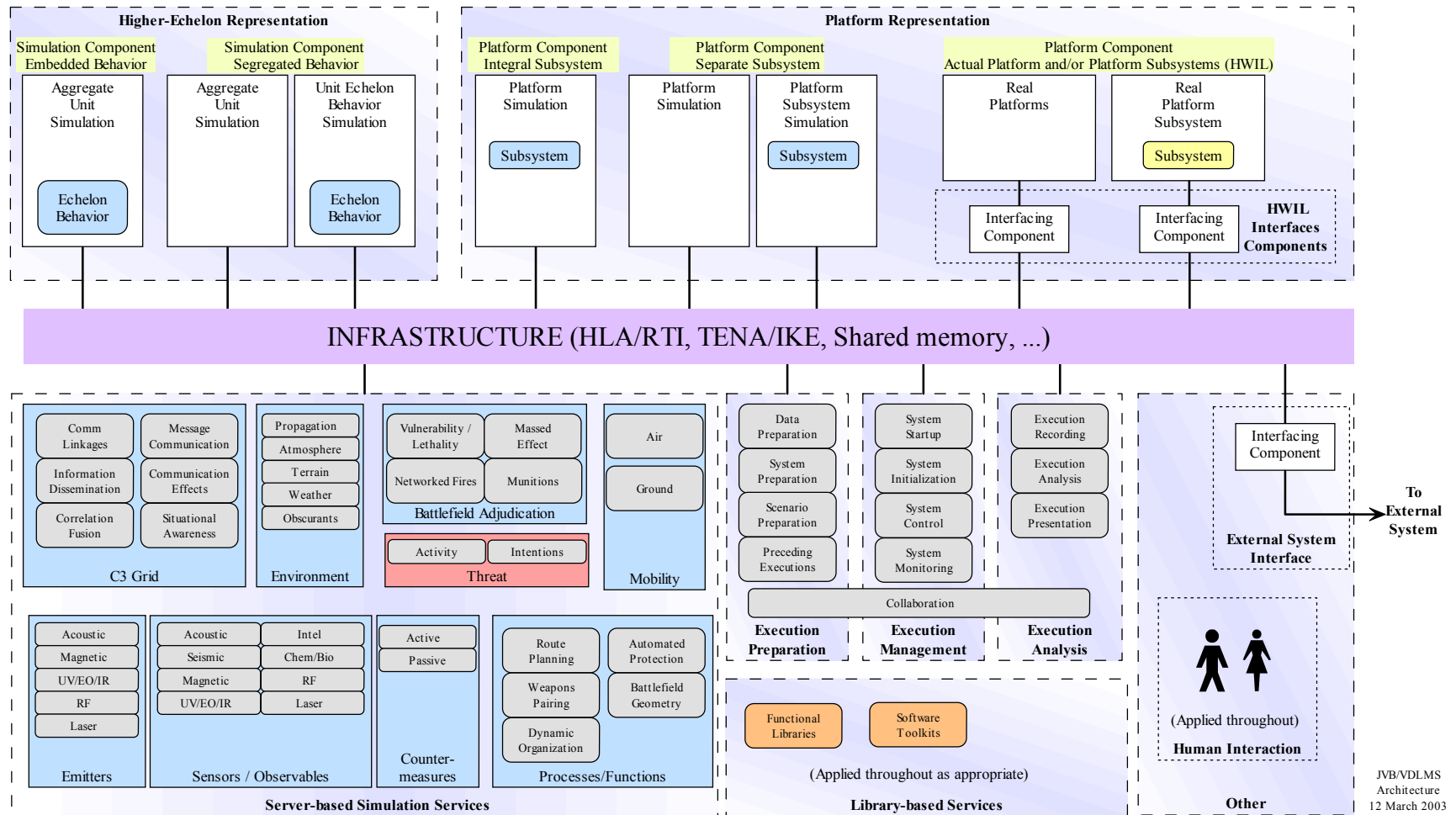
Figure 2. MATREX logical architecture (1, p 36).
