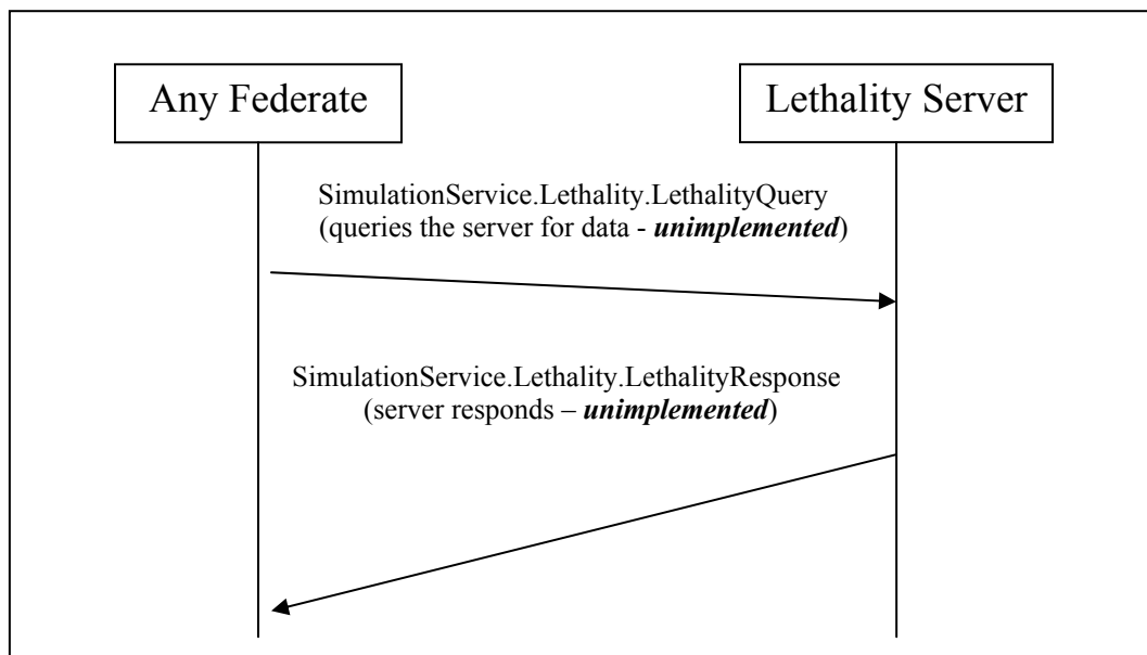
Figure 3. Query and response interaction.
