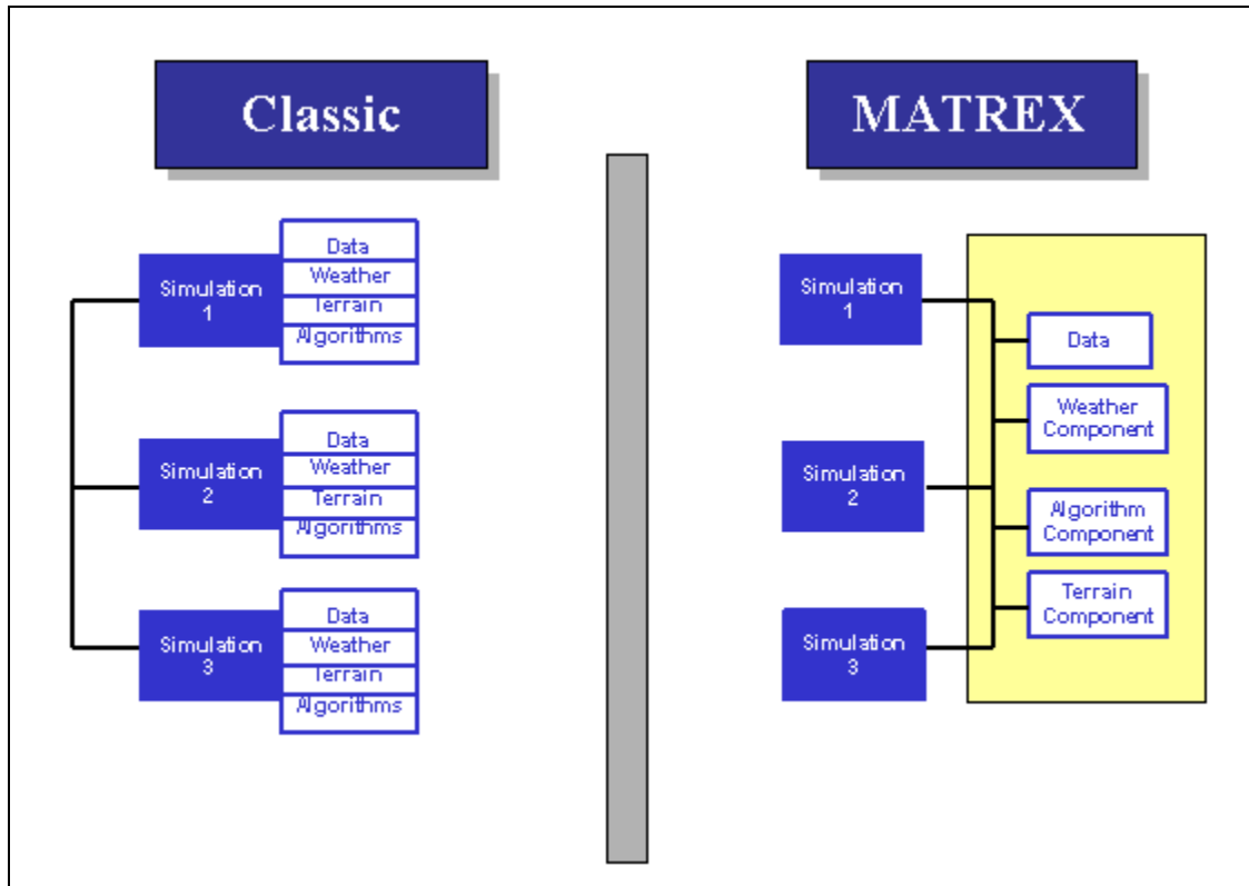
Figure 1. MATREX component architecture approach (1, p 30).
