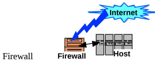
Replicated/Distributed System
