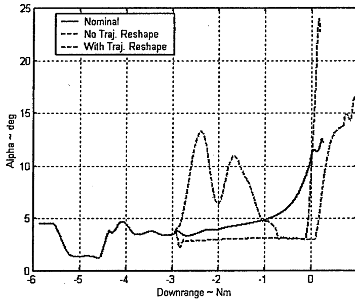
Figure 13. Angle-of-Attack History.
