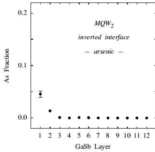
Figure 7. Indium and arsenic impurity profiles across the inverted heterojunction for MQW 2 .
