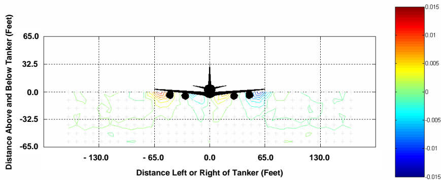
Roll Increment at 110 Ft Trail Position
