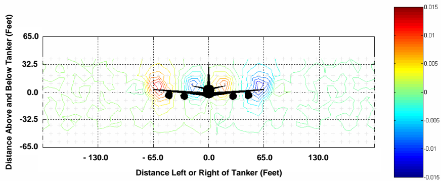
Roll Increment at 220 Ft Trail Position
