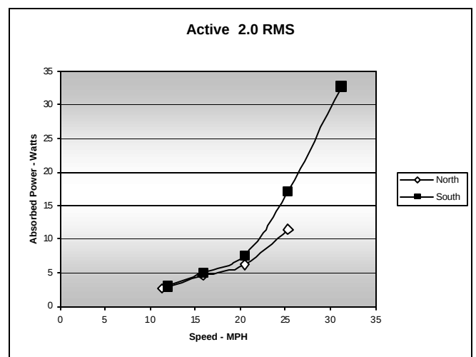
Figure 21 - Active 2.0 RMS
