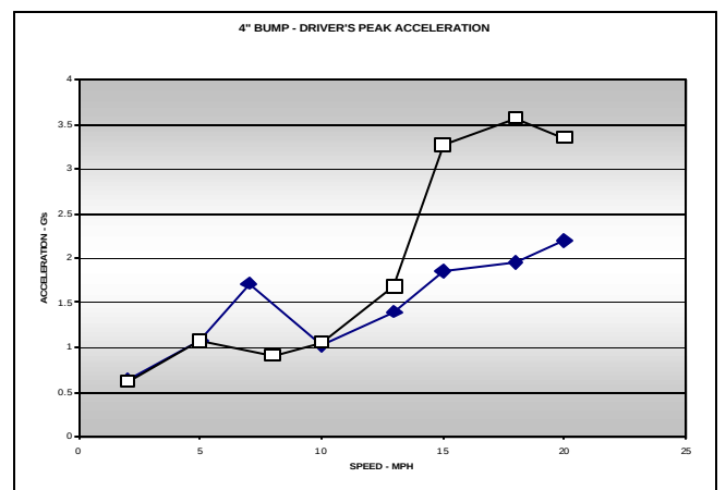
Figure 30 - 4" Bump Driver's Acceleration
