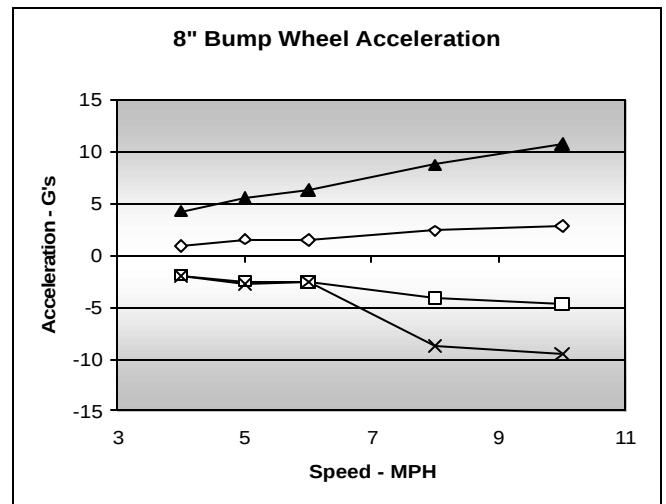
Figure 29 - 8" Bump Wheel Accelerations
