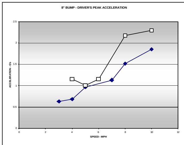
Figure 32 - 8" Driver's Acceleration
