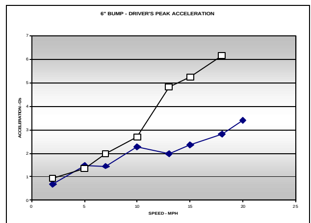
Figure 31 - 6" Driver's Acceleration
