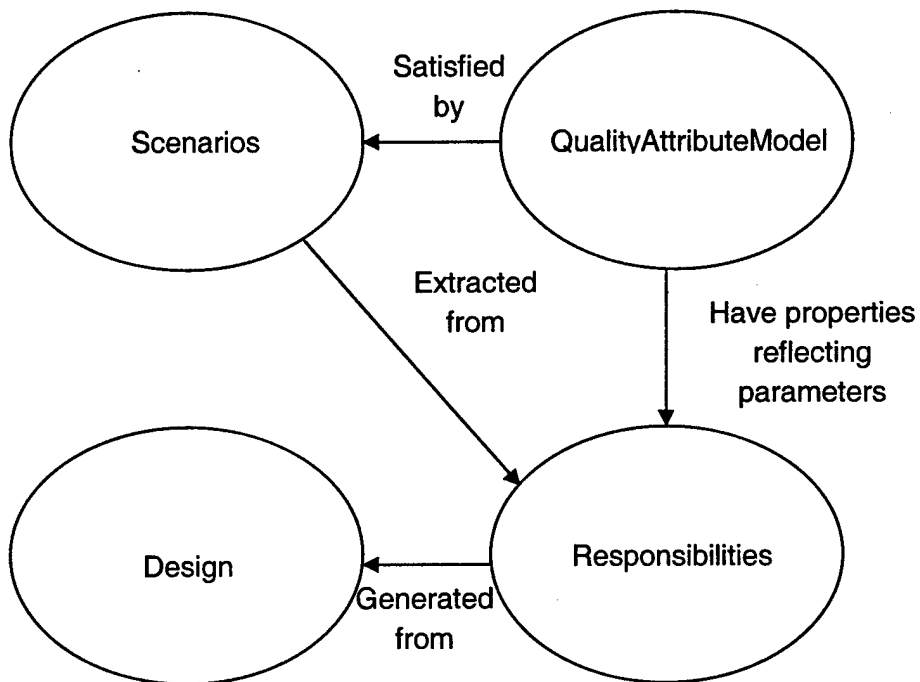
Figure 2: Key Concepts of ArchE and Their Relationships
