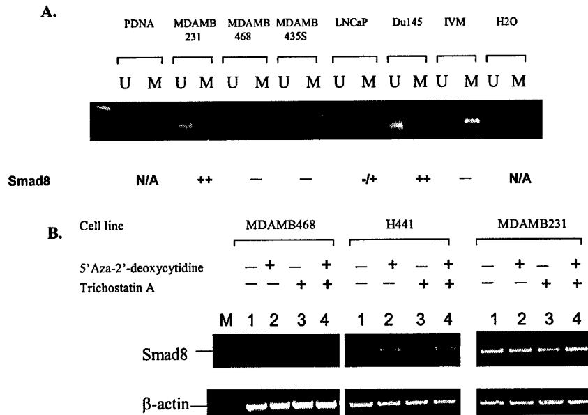
Figure 3. Epigenetic gene silencing of the SMAD8 gene by altered DNA methylation patterns. A. MSP (Methylation specific PCR) analysis of the CpG islands of intron 1 of the Smad8 gene in the indicated breast (MDAMB231, MDAMB468, MDAMB435S) and prostate (LNCaP, Du145) cancer cell lines that are either proficient (+) or deficient (-) in Smad8 expression. Placental DNA (PDNA) and in vitro methylated DNA (IVM) serve as negative and positive controls. Lanes U and lanes M indicate the presence of unmethylated and methylated templates, respectively. B. The indicated cell lines were treated with 1-5μM 5-AZA-dC for 7 days or with 300μM TSA for 24hrs. To assess the effect of both 5-AZA-dC and TSA simultaneously, cells were exposed sequentially for 7 days to 5-AZA-dC and subsequently to 300 μM TSA for an additional 24 hrs. Total RNA and genomic DNA were isolated and Smad8 expression and DNA hypermethylation were determined by RT-PCR and MSP analysis (data not shown), respectively.
