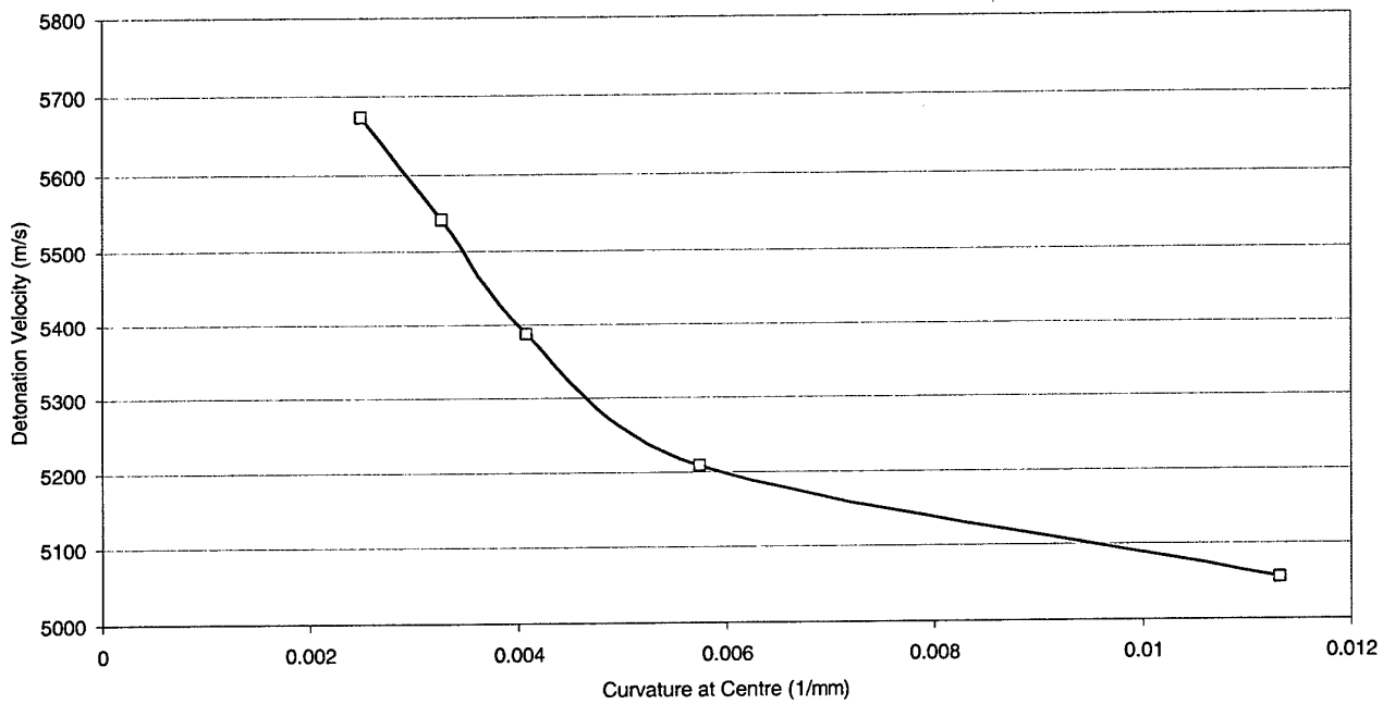
Figure 11 Detonation velocity of PBXW-115 (Aust) as a function of curvature at wave front centres
