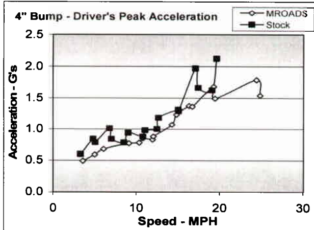
Figure 26 - 4" Bump Driver's Acceleration
