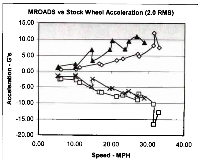
Figure 7- Comparison of Wheel Accelerations (2.0" RMS)
