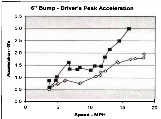
Figure 27 - 6" Bump Driver's Acceleration
