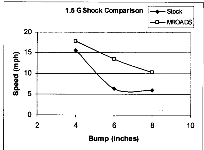
Figure 29 - 1.5 G Shock Comparison
