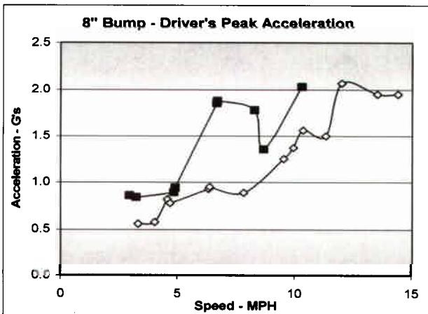
Figure 28 - 8" Bump Driver's Acceleration
