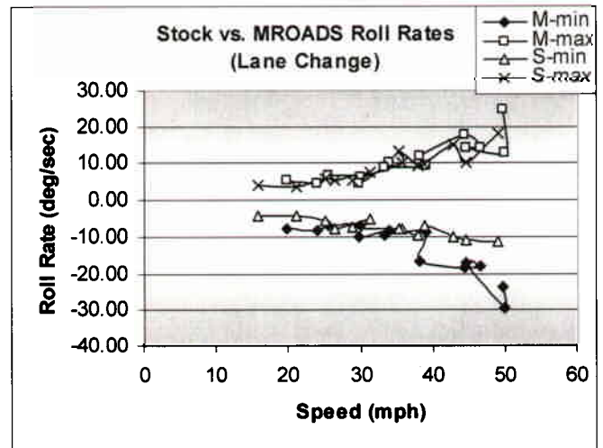
Figure 33 - Roll Rate (Lane Change)
