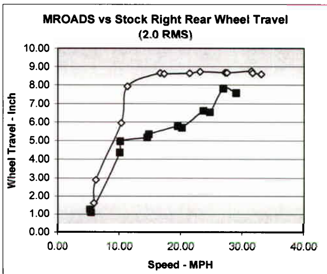
Figure 11 - Right Rear Wheel Travel (2.0" RMS)
