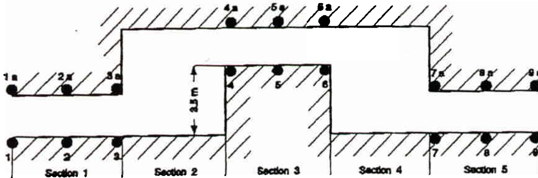
Figure A3 - Lane Change Layout
