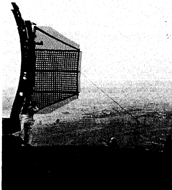
Members of the 609th Tactical Control Squadron, Bad Muender Air Station, set up an AN/TPS-43 at a deployed site in West Germany in support of Wintex '86 exercise. (USAF photo.)
