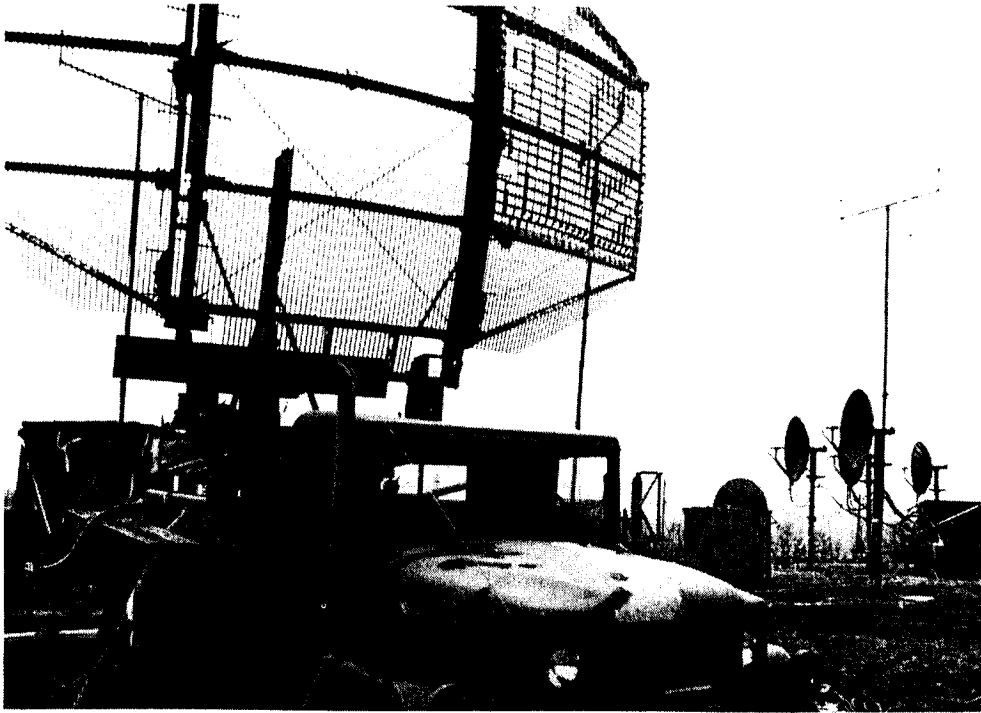
A TPS-43E radar configured on the bed of an M35 truck. TRC-97As (radio communication equipment) are set up on the right. (USAF photo.)
