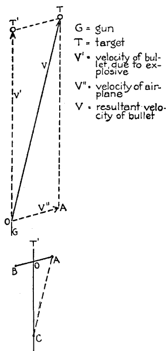
Figure 6. Principle of the Wind-Vane Sight
