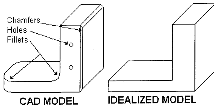
Figure 2: Model Idealization
