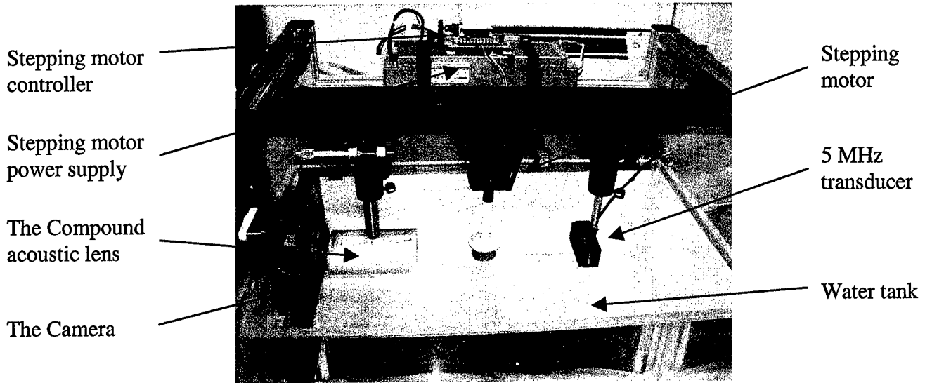
Figure 3. System components of the prototype transmission ultrasound system.
