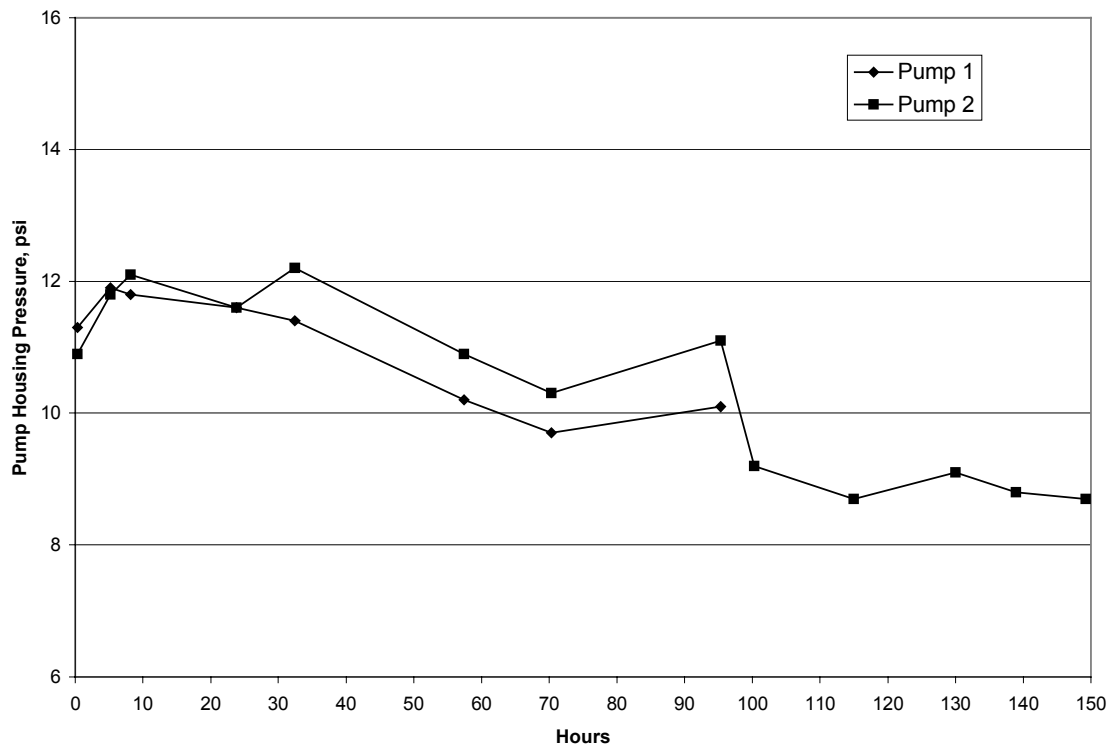
Figure A-4. Test 1 - Pump Housing Pressures
