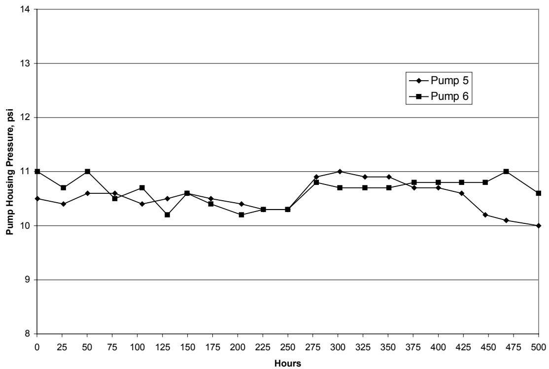
Figure A-12. Pump Test 3 - Pump Housing Pressures
