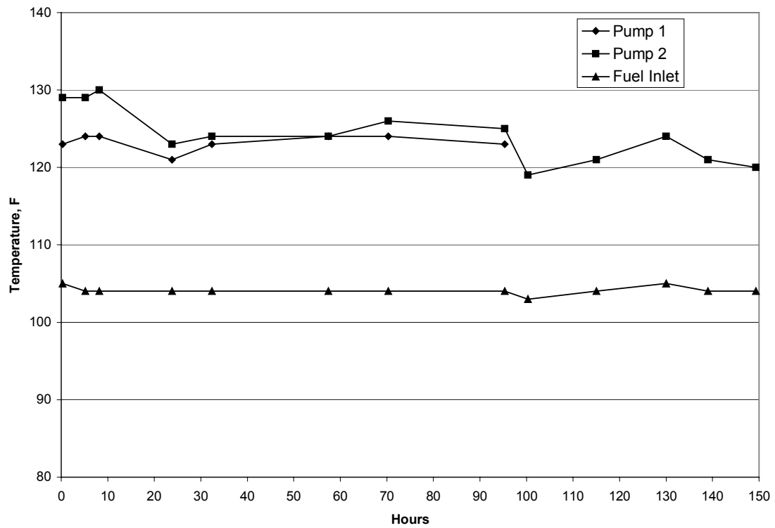
Figure A-2. Test 1 - Fuel Return and Inlet Temperatures
