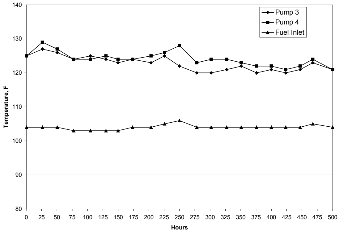
Figure A-6. Test 2 - Pump Return Fuel and Inlet Temperature
