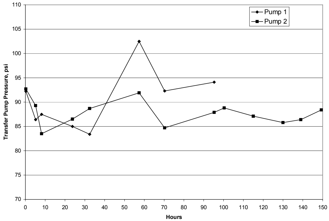
Figure A-3. Test 1 - Transfer Pump Pressures
