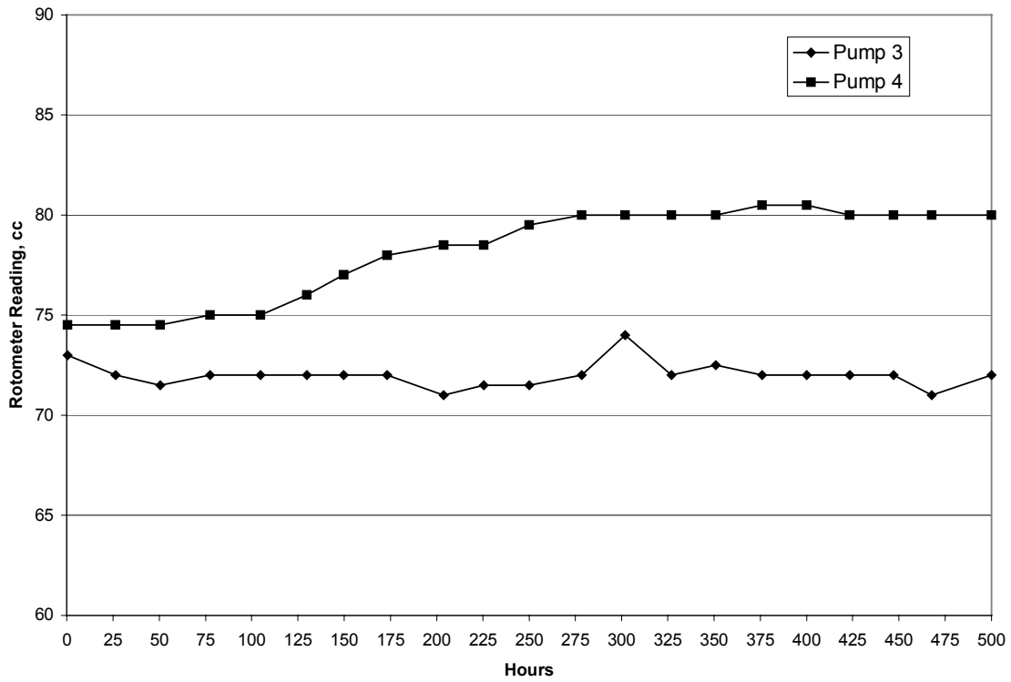
Figure A-5. Test 2 - Rotameter Readings
