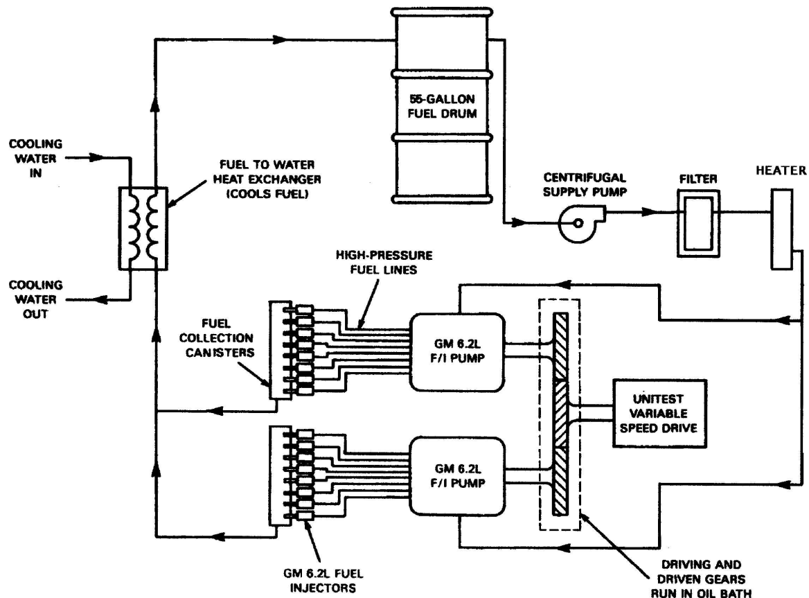
Figure 4. Fuel System Schematic
