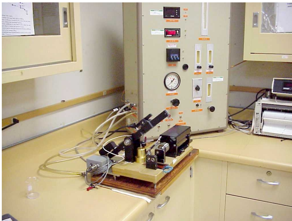
Figure 1. Instrument for BOCLE and Scuffing Load BOCLE Tests
