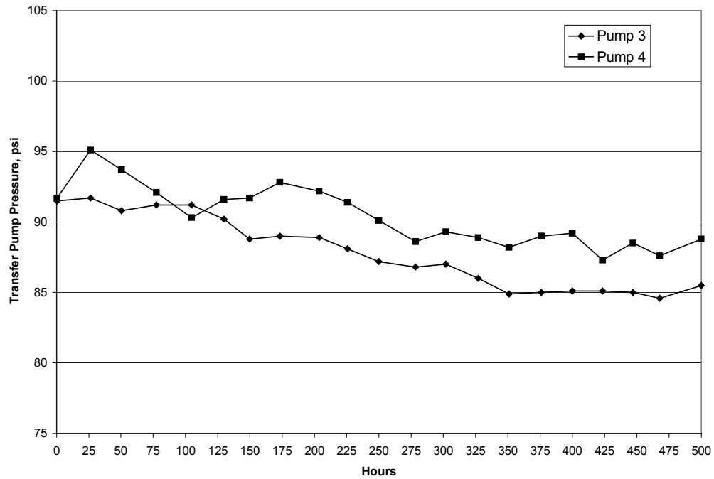
Figure A-7. Test 2 - Transfer Pump Pressures
