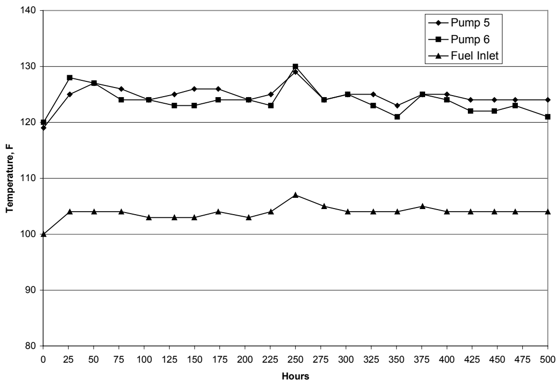
Figure A-10. Test 3 - Pump Return Fuel and Inlet Temperatures
