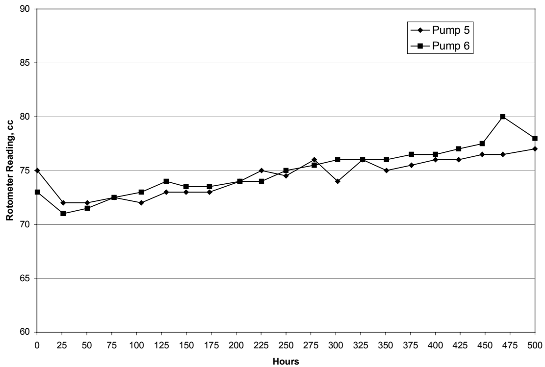
Figure A-9. Pump Test No. 3 - Rotameter Readings
