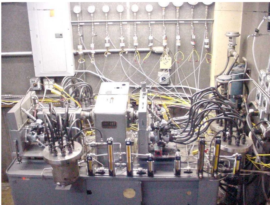
Figure 5. Pump Stand
