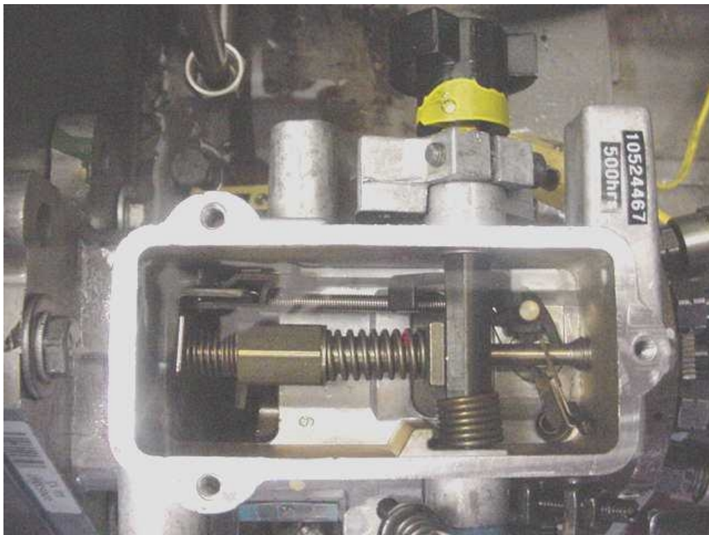
Figure 18. Test 2 Pump 4: Pump Chamber
