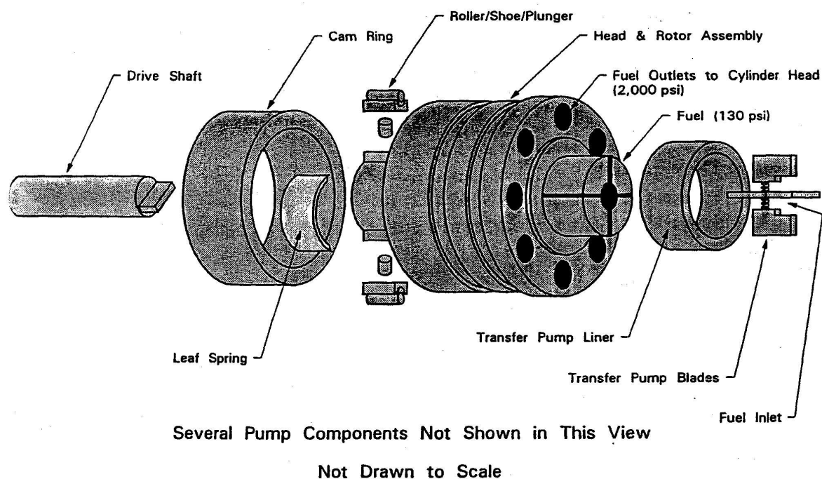
Figure 3. Schematic Diagram of Principal Pump Components
