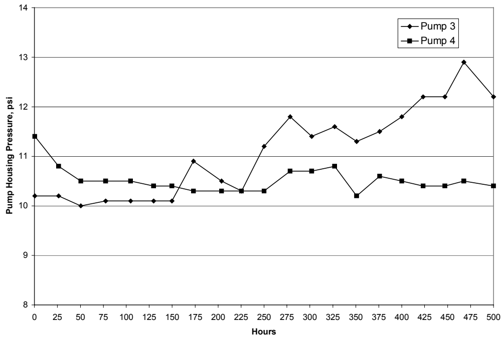
Figure A-8. Test 2 - Pump Housing Pressures
