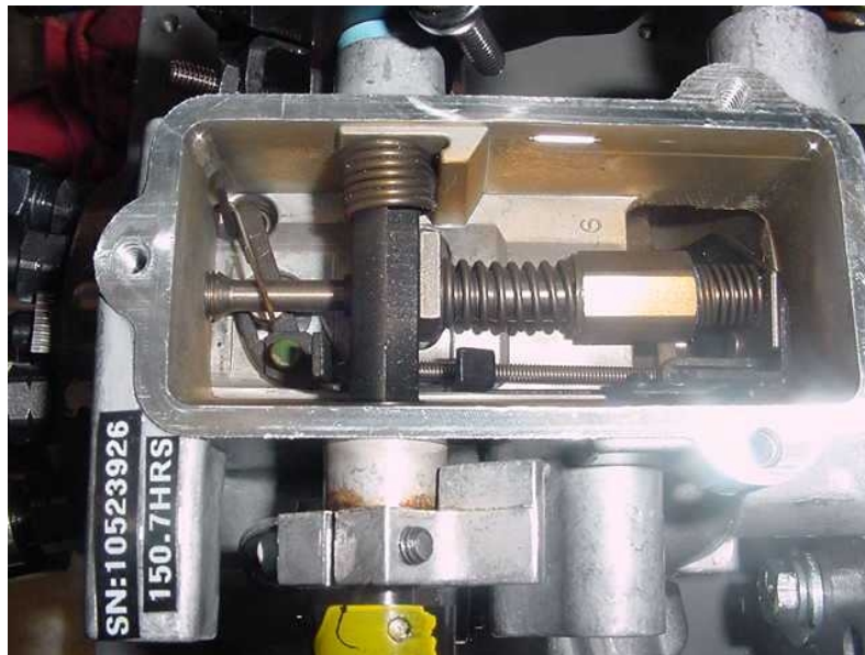
Figure 8. Test 1 Pump 2: Debris Free Pump Chamber
