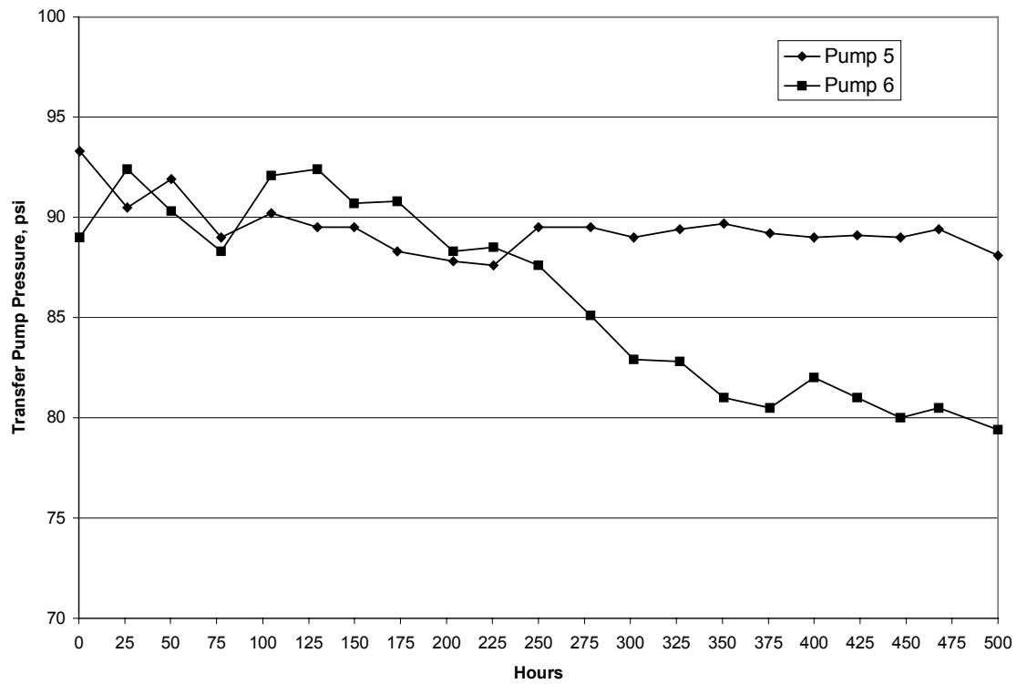
Figure A-11. Test 3 - Transfer Pump Pressures
