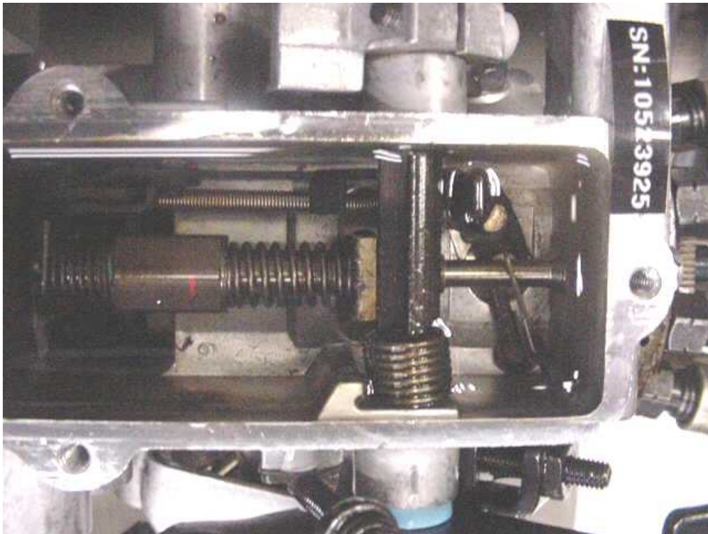
Figure 6. Test 1 Pump 1: Pump Chamber Wear Debris
