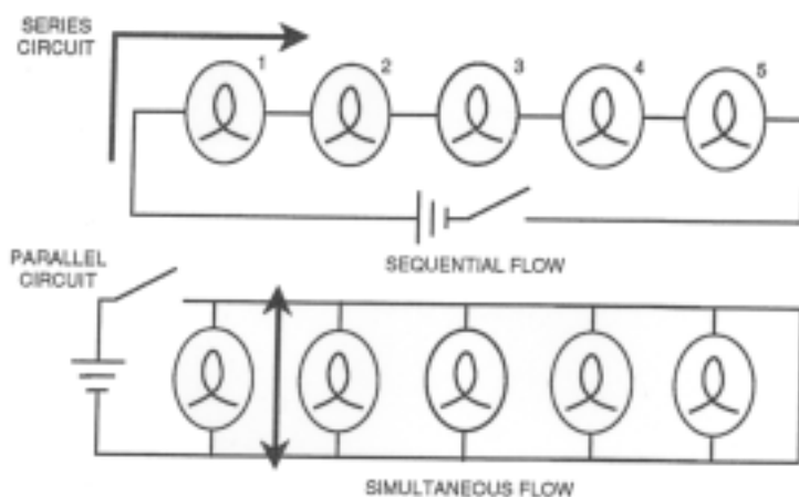
Figure 1. Comparison of series circuit with sequential flow to parallel circuit with simultaneous flow.
