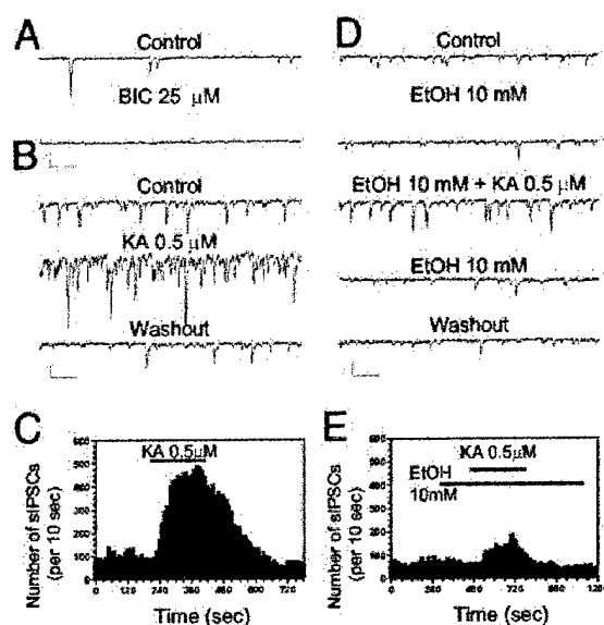
Fig. 1. EtOH inhibits the KA-R-mediated increase of sIPSC frequency in CA1 pyramidal neurons. (A) sIPSCs are fully blocked by the GABA _A -R antagonist, bicuculline (BIC; 25 \mu\text{M} ). (B and C) Bath application of KA (0.5 \mu\text{M} ) for 3.5 min, in the presence of GYKI 53655 (30 \mu\text{M} ) and DL-AP5 (100 \mu\text{M} ), induced a robust and reversible sIPSC frequency increase. (D and E) EtOH (10 mM) did not affect either the basal amplitude or frequency of sIPSCs, but reduced the increase in frequency induced by KA-R-activation. (Scale bars: 100 pA and 250 ms.)
