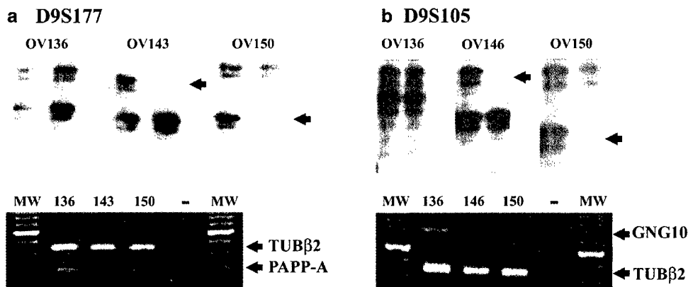
Figure 3 Representative examples of LOH and corresponding LOE. For both D9S177 (a) and D9S105 (b), one example of intact alleles without downregulation of gene expression is shown, along with two examples of LOH showing concurrent LOE. Scored LOH is indicated with arrows
