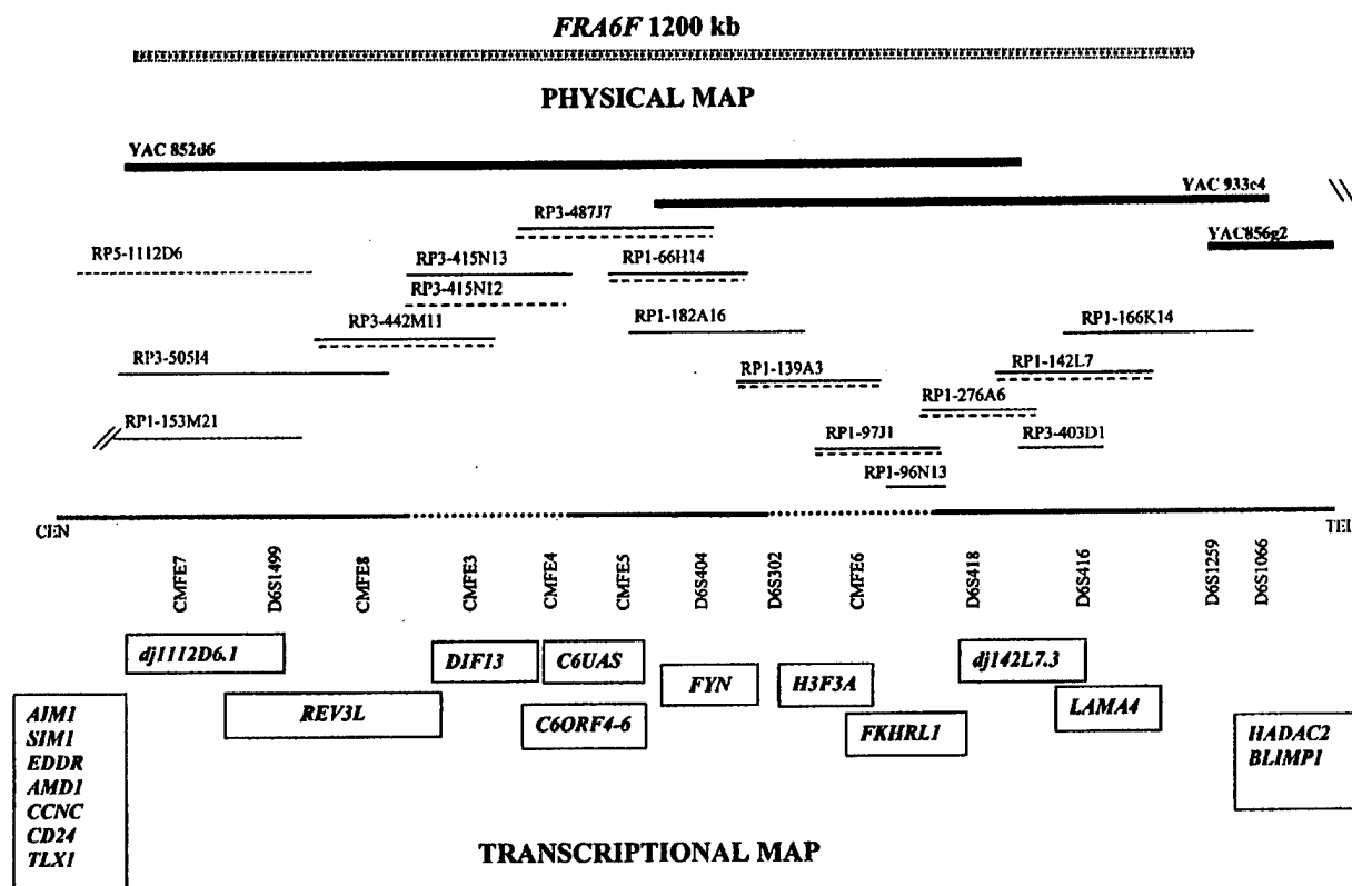
Figure 1 Physical and transcriptional map of the FRA6F region. The physical map and the whole region of breaking are reported in the top part of the figure with the markers distributed along the region. Dotted lines indicate the two hot-spots of breaking, revealed by FISH experiments with PAC probes. Thick bold lines represent the YAC clones used for initial FRA6F localization. PAC clones used in FISH experiments are shown in the figure with plain lines. PAC clones subjected to sequence analysis are indicated with dashed lines. PAC clones marked with both continuous and dashed lines have been used for FISH experiments and sequence analysis. The transcriptional map of FRA6F is shown in the lower part of the figure with genes distributed in the regions proximal to, within and distal to FRA6F
