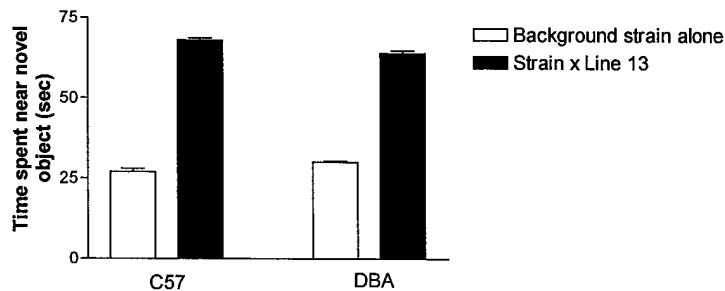
Figure 5: Entries into center and time near the novel object in control strains (C57 or DBA, open bars) compared to the 5HT3 receptor over-expressing gene on the two inbred strain backgrounds (C57 and DBA, closed bars). A significant decrease in anxious behavior was seen in the C57Bl mice with the 5HT3 receptor over-expression indicated by the increase center entries. Interestingly the 5HT3 receptor over-expression did significantly increase time spent with novel object for the DBA mice. Indicating the 5HT3 receptor may play a role in inquisitive behavior .
