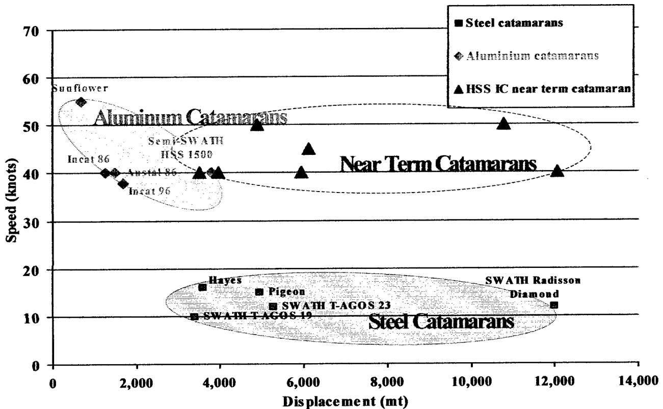
Figure 9 Catamaran Technology
