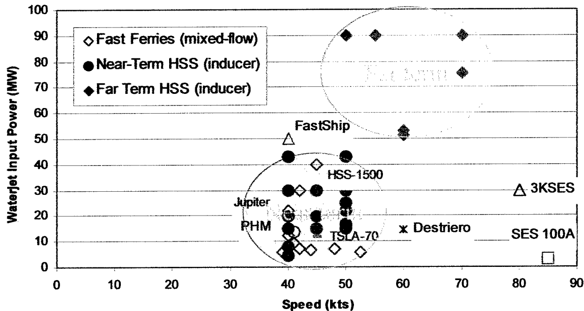
Figure 13 Waterjet Technology
