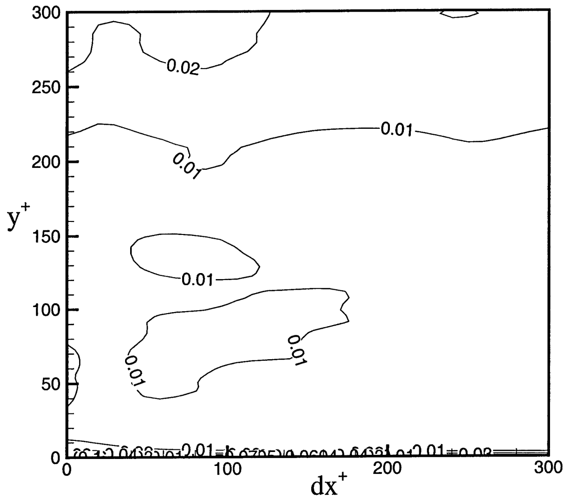
Figure 2: Same as figure 1a, but for the \phi_{33,33}(r_1)
