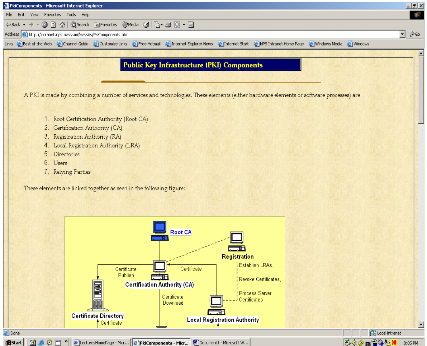
Figure 31. PKI Components
