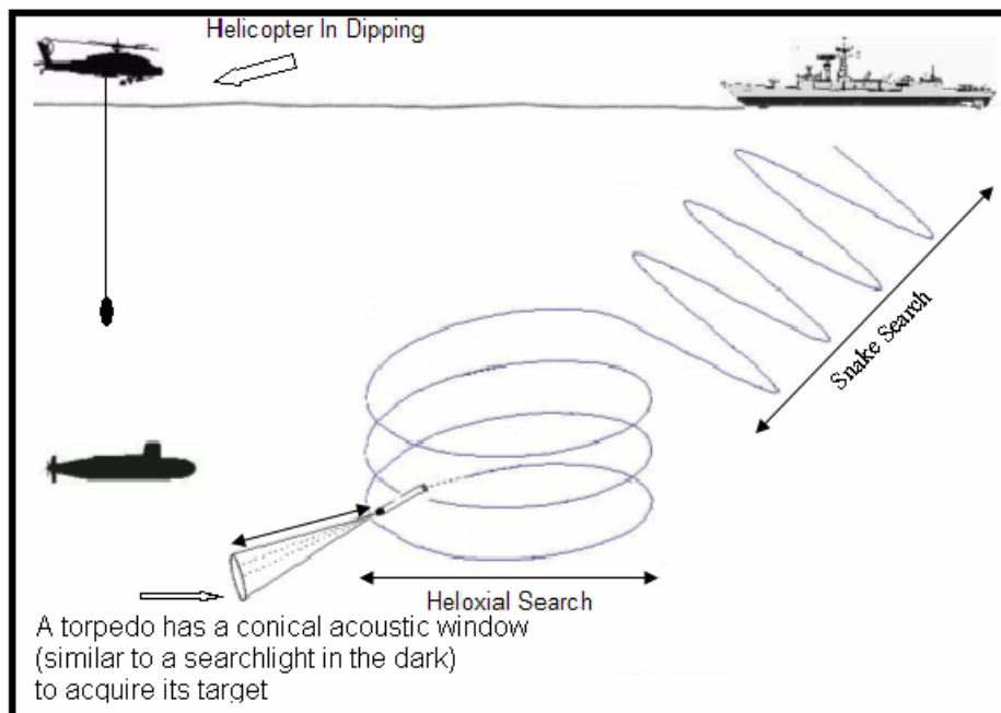
Figure 4. Active Homing Torpedo Search Pattern
