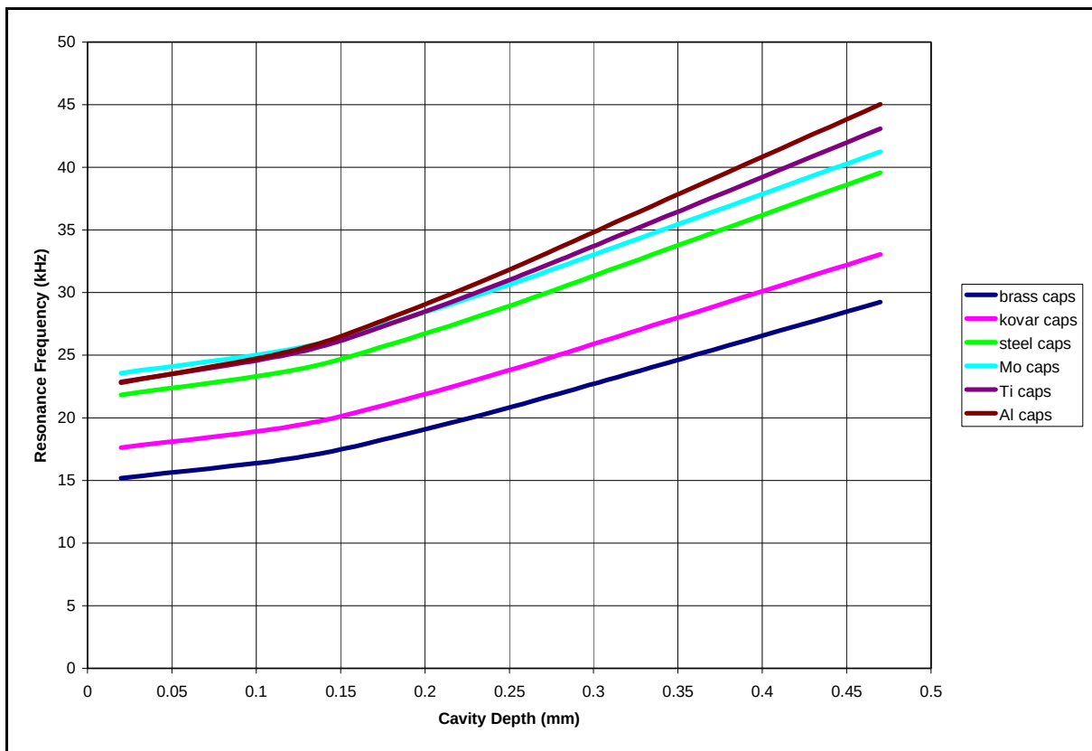
Figure 5. Resonance frequency (in-air) vs. cavity depth for various materials 8
