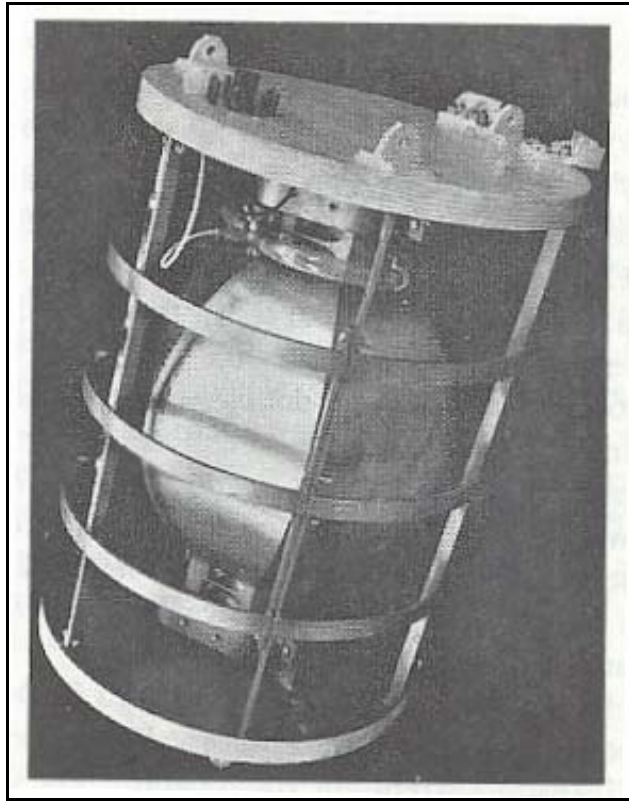
Figure 2. Underwater flextensional transducer from Ref [4] 2
