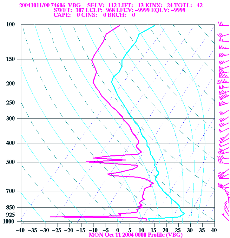
Figure 173. Thermosonde 11, launch time 0413Z 210CT01.
