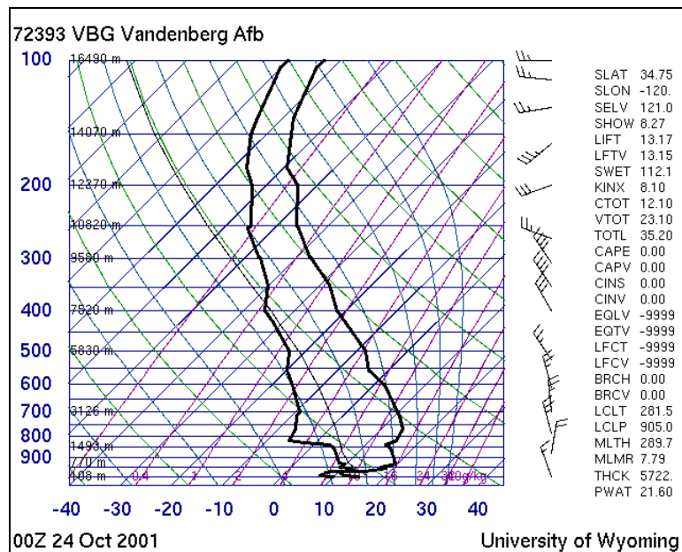
Figure 142. Vandenberg AFB, 00Z 240CT01.
