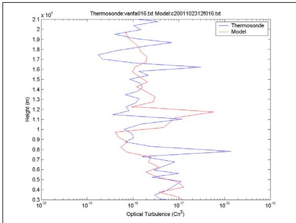
Figure 35. C_n^2 profile comparison for 240CT01 04Z.
