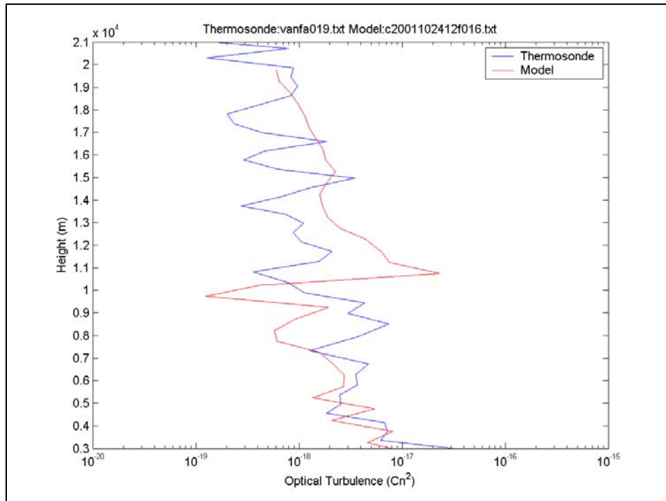
Figure 38. C_n^2 profile comparison for 250CT01 04Z.
