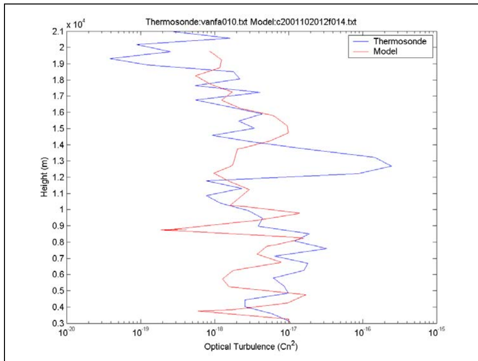
Figure 30. C_n^2 profile comparison for 210CT01 02Z.
