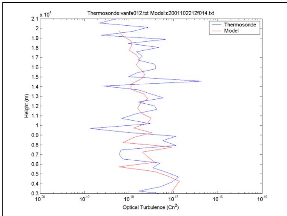
Figure 32. C_n^2 profile comparison for 230CT01 02Z.
