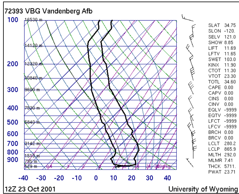
Figure 141. Vandenberg AFB, 12Z 230CT01.
