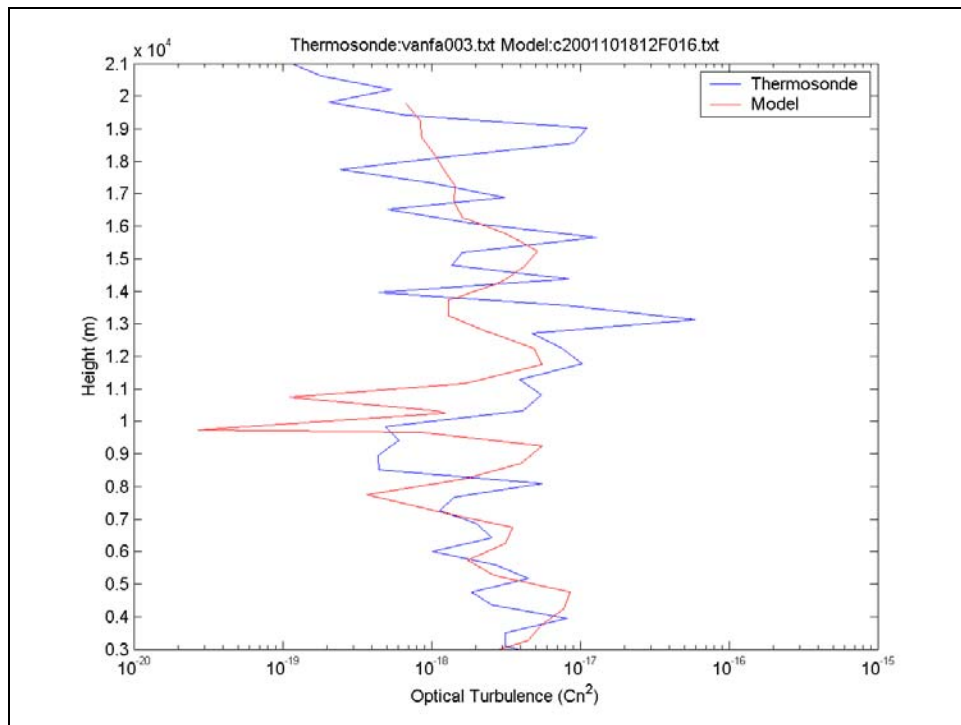
Figure 26. C_n^2 profile comparison for 190CT01 04Z.
