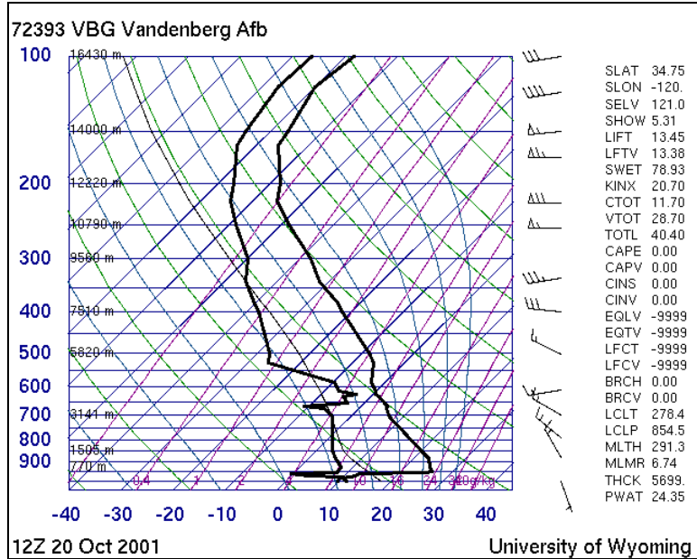
Figure 135. Vandenberg AFB, 12Z 20OCT01.
