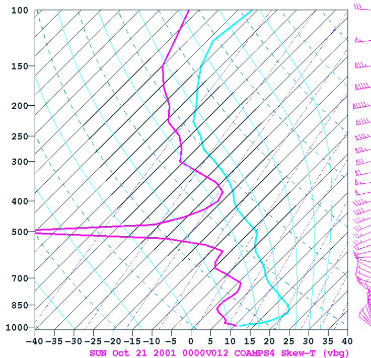
Figure 152. COAMPS forecast for 00Z, 210CT01.
