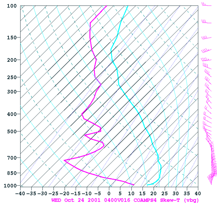
Figure 160. COAMPS forecast for 04Z, 24OCT01.
