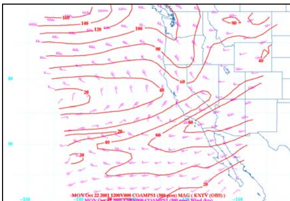
Figure 124. COAMPS 300 mb analysis valid 12Z 220CT01.
