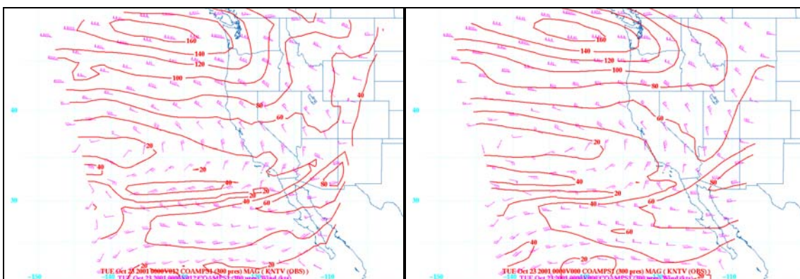
Figure 125. COAMPS 300 mb forecast (left) and analysis (right) valid for 00Z, 230CT01.
