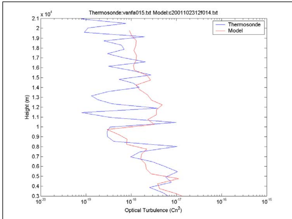
Figure 34. C_n^2 profile comparison for 240CT01 02Z.
