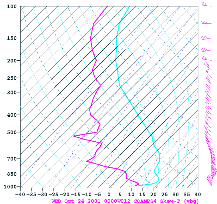
Figure 158. COAMPS forecast for 00Z, 24OCT01.
