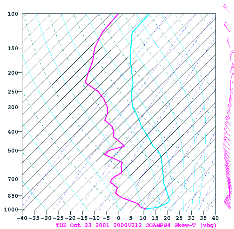
Figure 155. COAMPS forecast for 00Z, 23OCT01.
