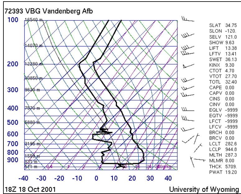
Figure 131. Vandenberg AFB, 18Z 18OCT01.
