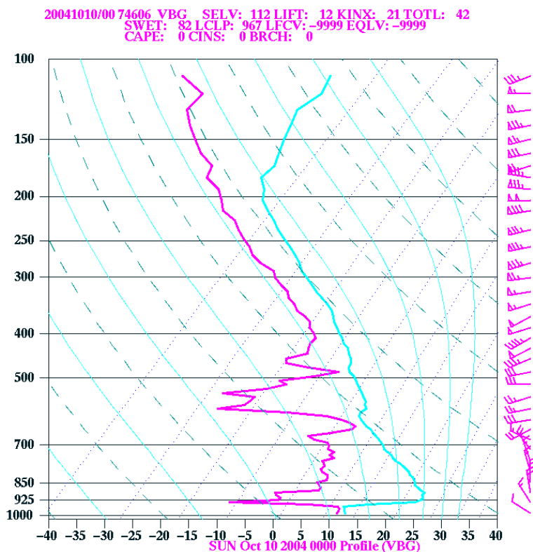
Figure 172. Thermosonde 10, launch time 0235Z 210CT01.
