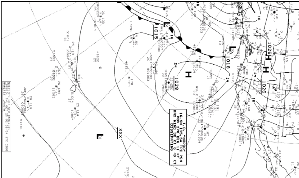
Figure 59. NCEP/MPC 00Z Surface Analysis, 250CT01.
