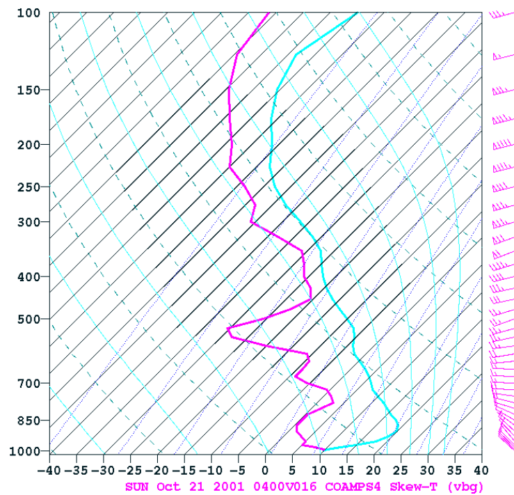
Figure 154. COAMPS forecast for 04Z, 210CT01.
