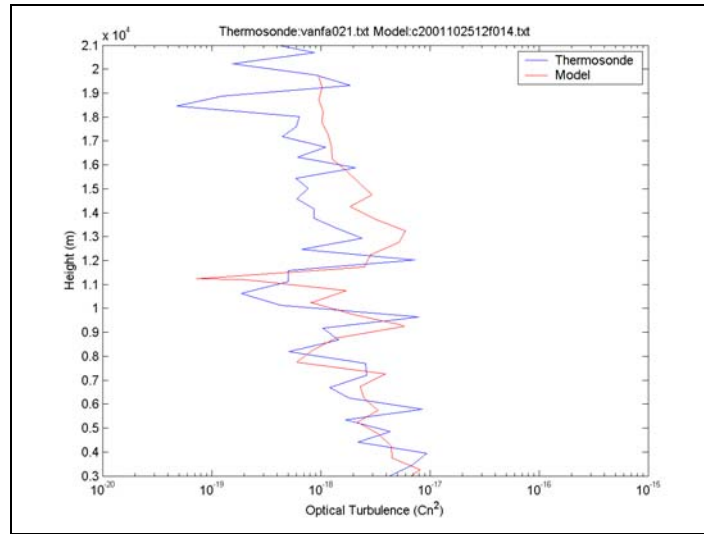
Figure 39. C_n^2 profile comparison for 260CT01 02Z.
