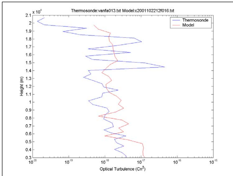
Figure 33. C_n^2 profile comparison for 230CT01 04Z.
