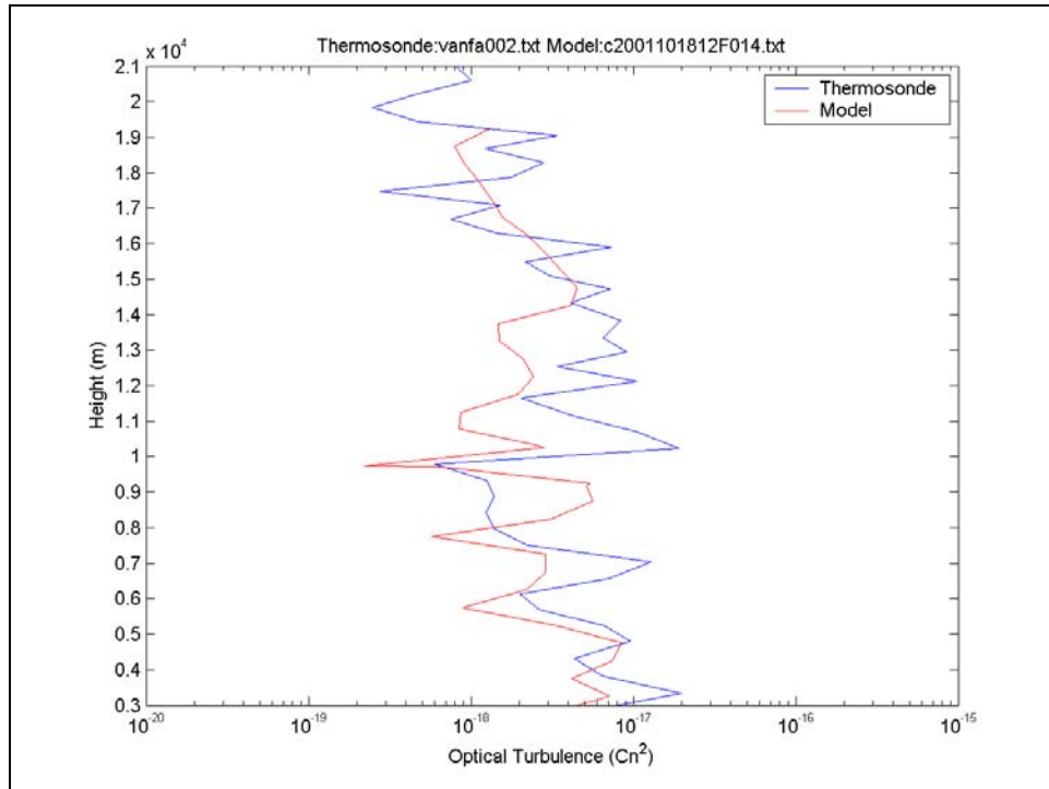
Figure 25. C_n^2 profile comparison for 190CT01 02Z.
