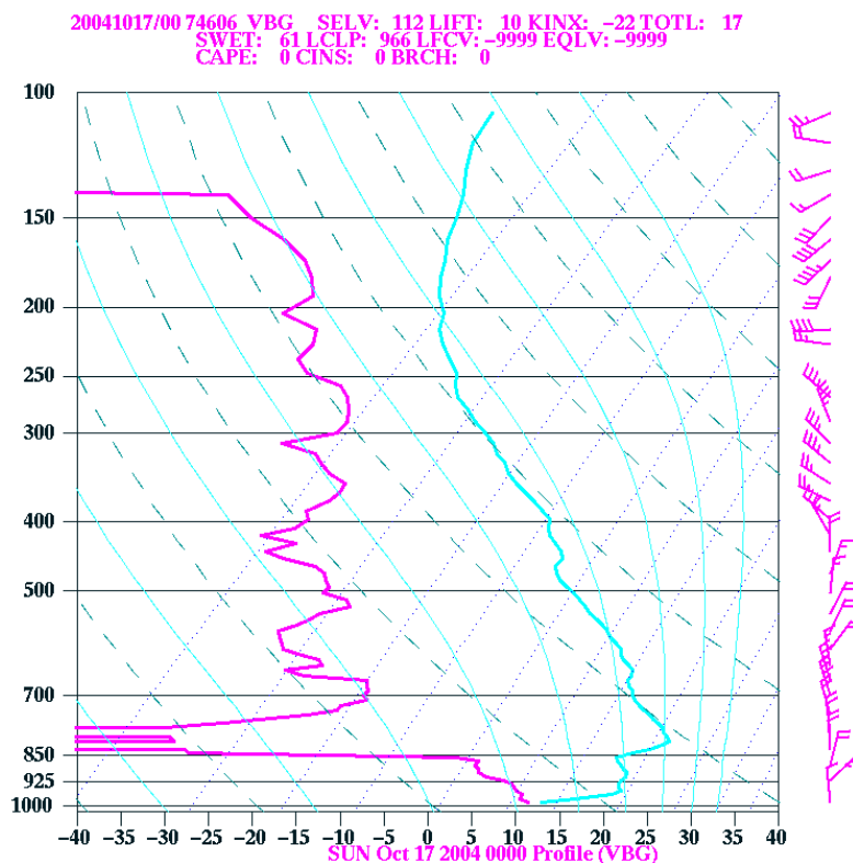
Figure 178. Thermosonde 17, launch time 0430Z 240CT01.
