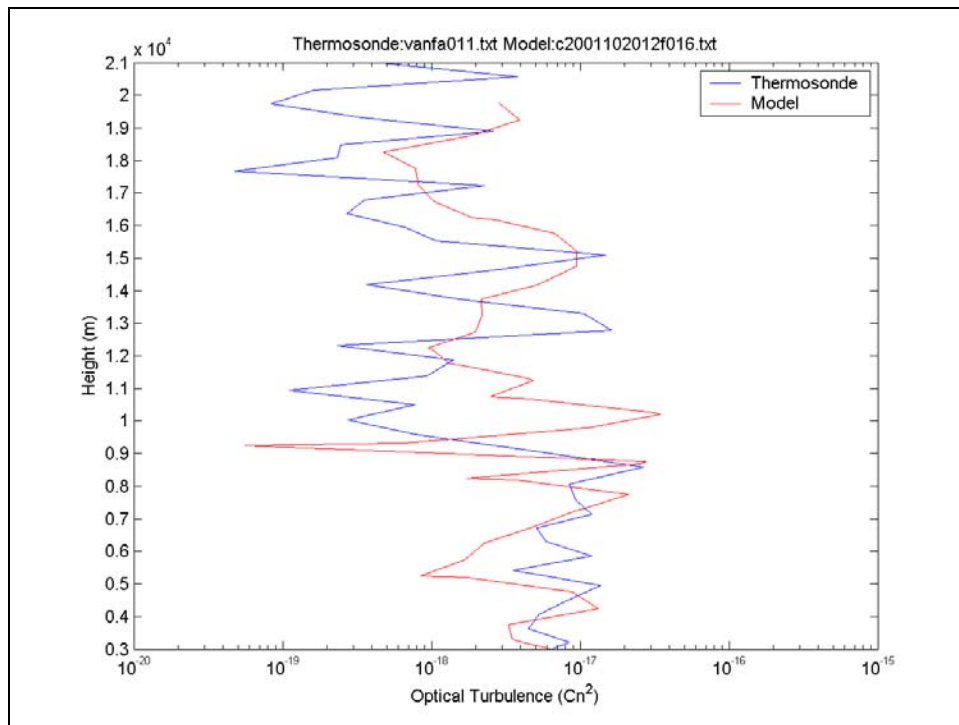
Figure 31. C_n^2 profile comparison for 210CT01 04Z.
