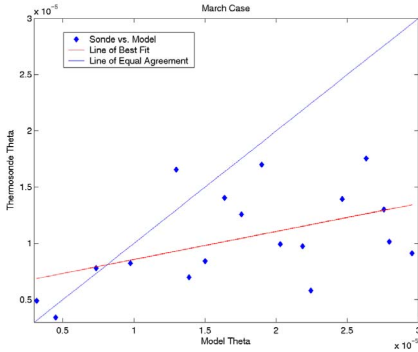
Figure 42. \theta_o Scatter plot results for COAMPS and thermosonde C_n^2 values for March 2002.
