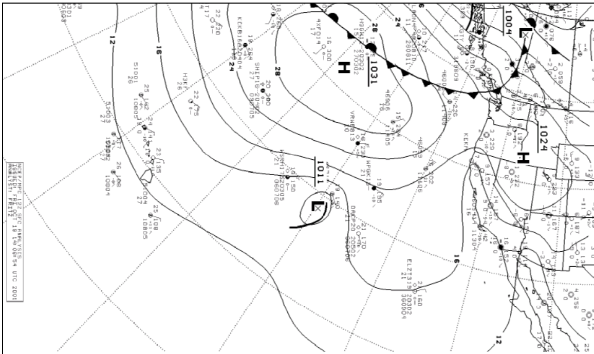
Figure 48. NCEP/MPC 12Z Surface Analysis, 190CT01.
