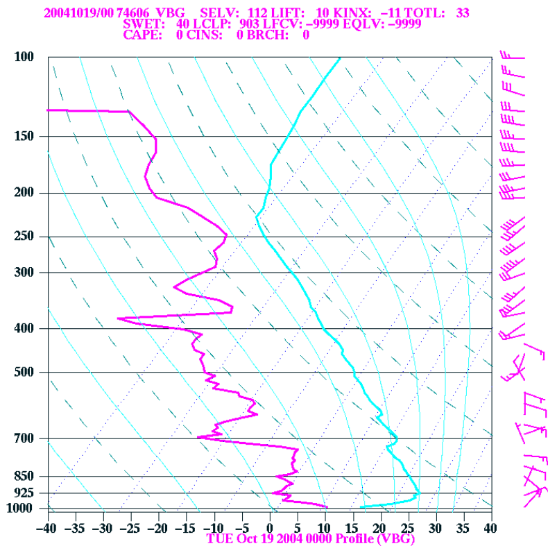
Figure 180. Thermosonde 19, launch time 0253Z 250CT01.
