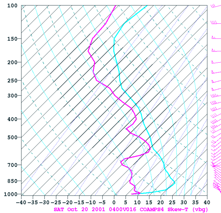
Figure 150. COAMPS forecast for 04Z, 200CT01.
