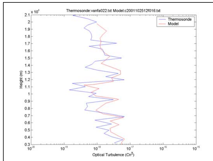
Figure 40. C_n^2 profile comparison for 260CT01 04Z.
