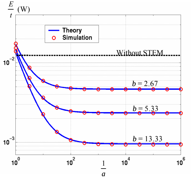
Figure 8 – Relative energy savings of STEM versus the predominance of the transfer state
