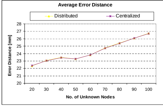
Figure 14: Quality of localizations a unknown nodes increase
