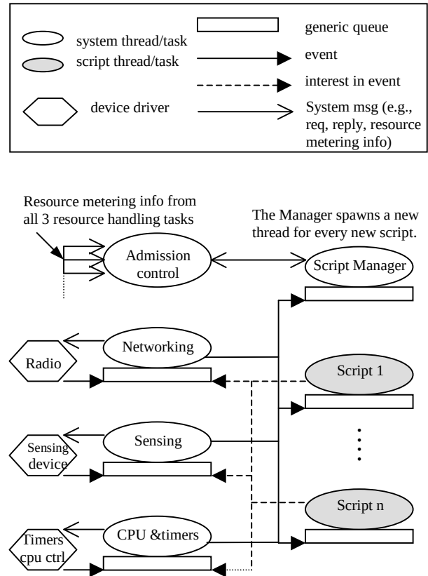
Figure 6: Abstracted view of SensorWare's run-time environment
