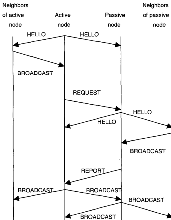
Fig. 2. Protocol message exchanges
