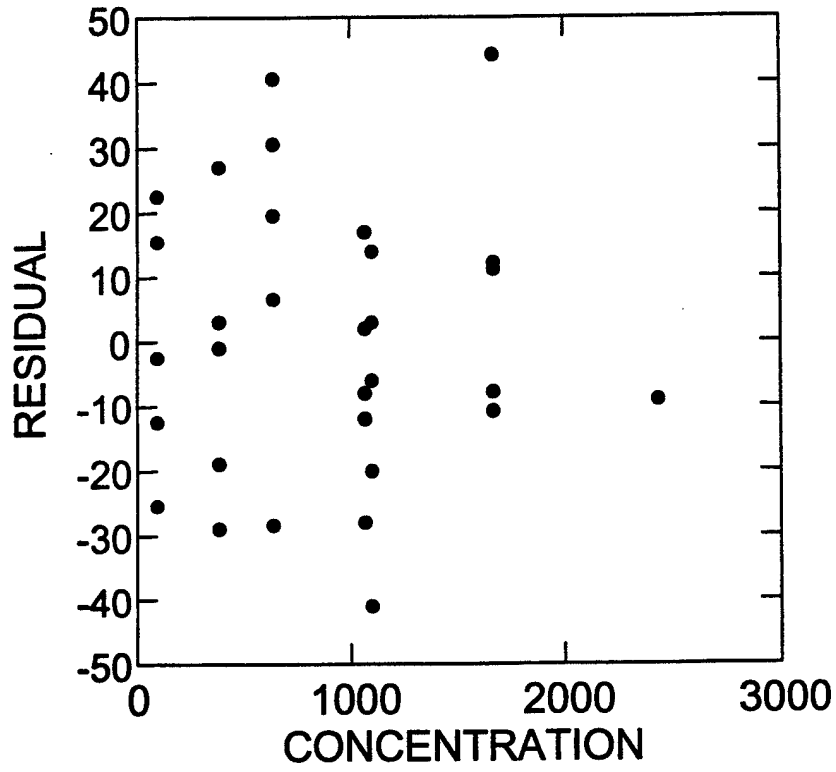
Residuals for Mn
