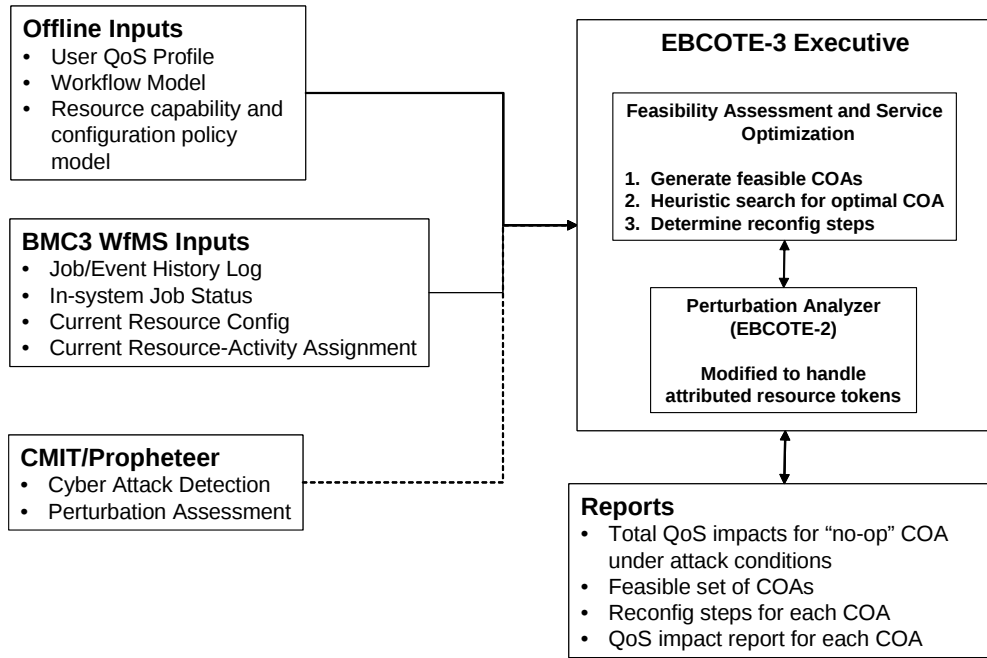
Figure 2. System architecture for EBCOTE-3.
