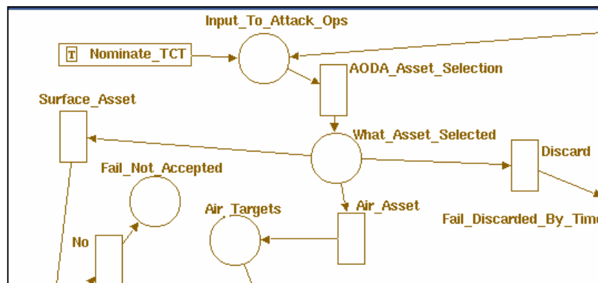
Figure 4. Target candidates may be prosecuted by surface or air assets depending on the result of the AODA Asset Selection task.
