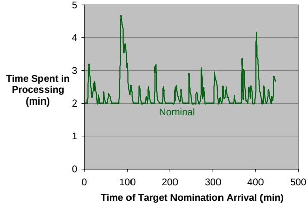
Figure 9. Service Times Under Nominal Conditions.
