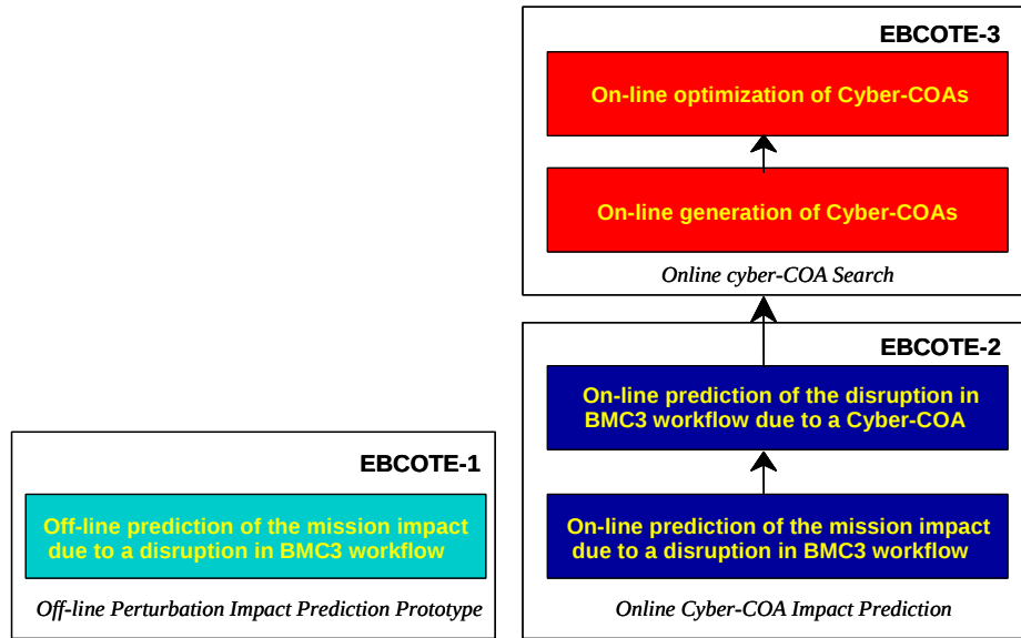
Figure 1. Three research stages in the evolution of the EBCOTE system.
