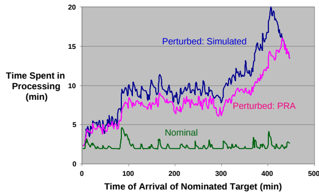
Figure 11. Service Times When the DOS Attack Blocks Database Access Requests
