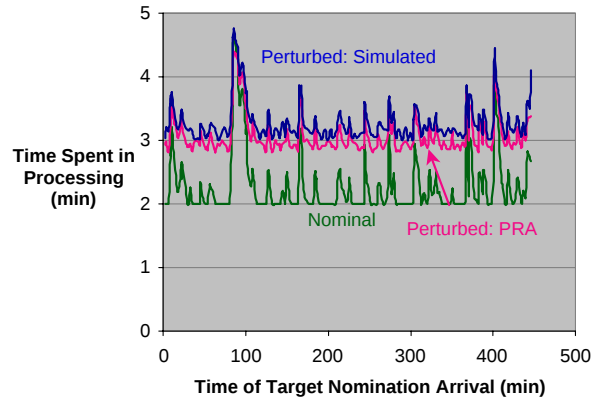
Figure 10. Service Times When the DOS Attack Simply Retards Processing
