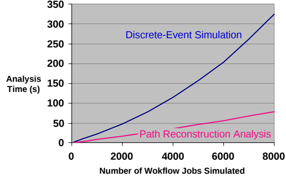
Figure 12. Runtime vs. Workflow Size for Monte-Carlo Simulation and PRA
