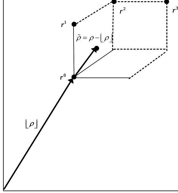
Figure 15. We can find a selection set for the fractional part of our continuous solution, without loss of generality.
