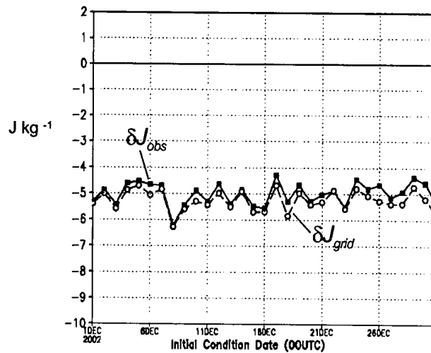
Figure 8: Gradient test comparison for \delta J_{obs} (solid line) and \delta J_{grid} (dash line) for Dec 2002. Costfunction J is NOGAPS forecast error ( e_{24} - e_{30} , J \text{ kg}^{-1} ) in the global domain. \delta J_{obs} and \delta J_{grid} are defined in Section 3.3.
