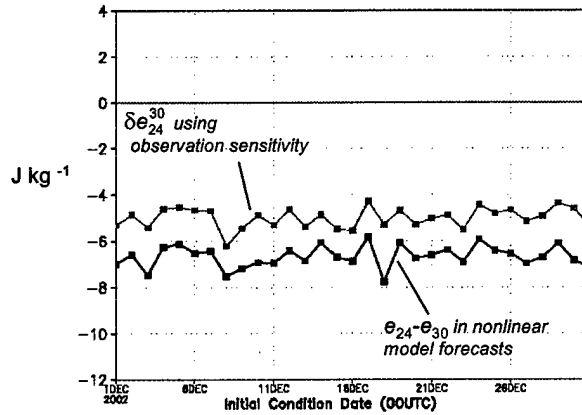
Figure 10: Time series of e_{24} - e_{30} (dark solid line) in NOGAPS forecasts and corresponding adjoint-based observation impact estimate \delta e_{24}^{30} (grey solid line) calculated using Eq. 16 in the global domain with no moisture observations in December 2002.
