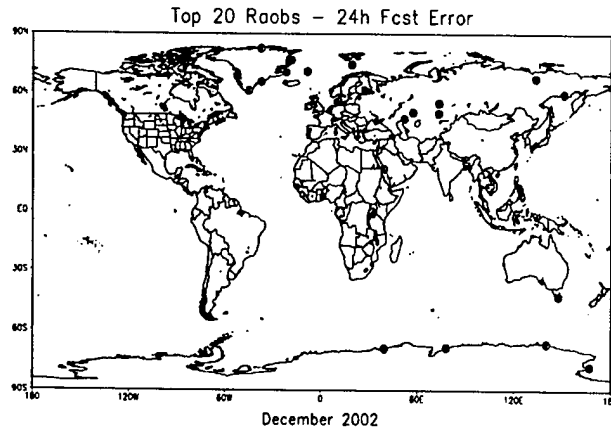
Figure 13: Twenty rawinsonde observing stations that produce the largest observation impact \delta e_{24}^{30} , representing reductions of e_{24} - e_{30} in the global domain, due to observations assimilated at 00UTC in December 2002.
