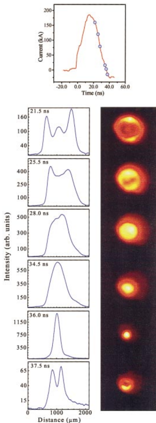
FIG. 3. (Color) Sequence of time resolved pinhole camera images of the plasma for the same discharge conditions of Fig. 2 taken using only a 1\text{ }\mu\text{m} thick C filter. The filter transmits photons below 3 nm and also in the range between 4.5 and 10 nm.
