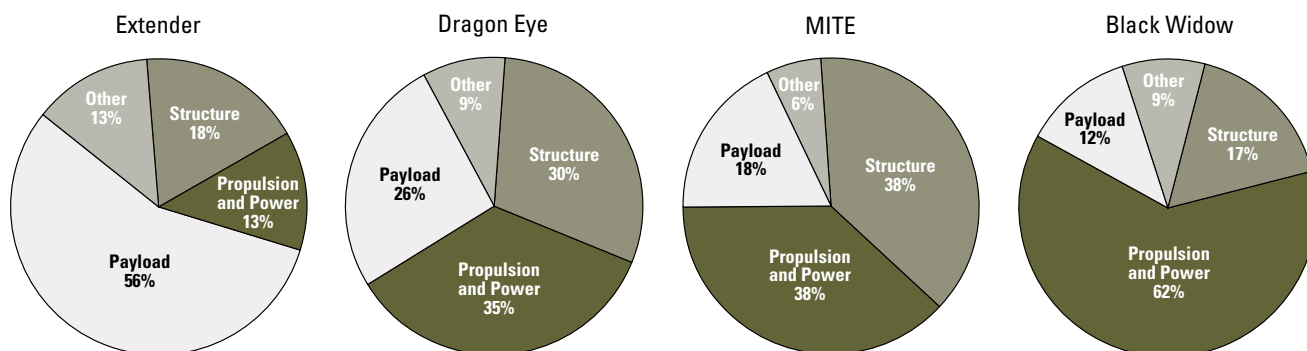
Figure 1. Weight Budgets for 20-Minute Flight
