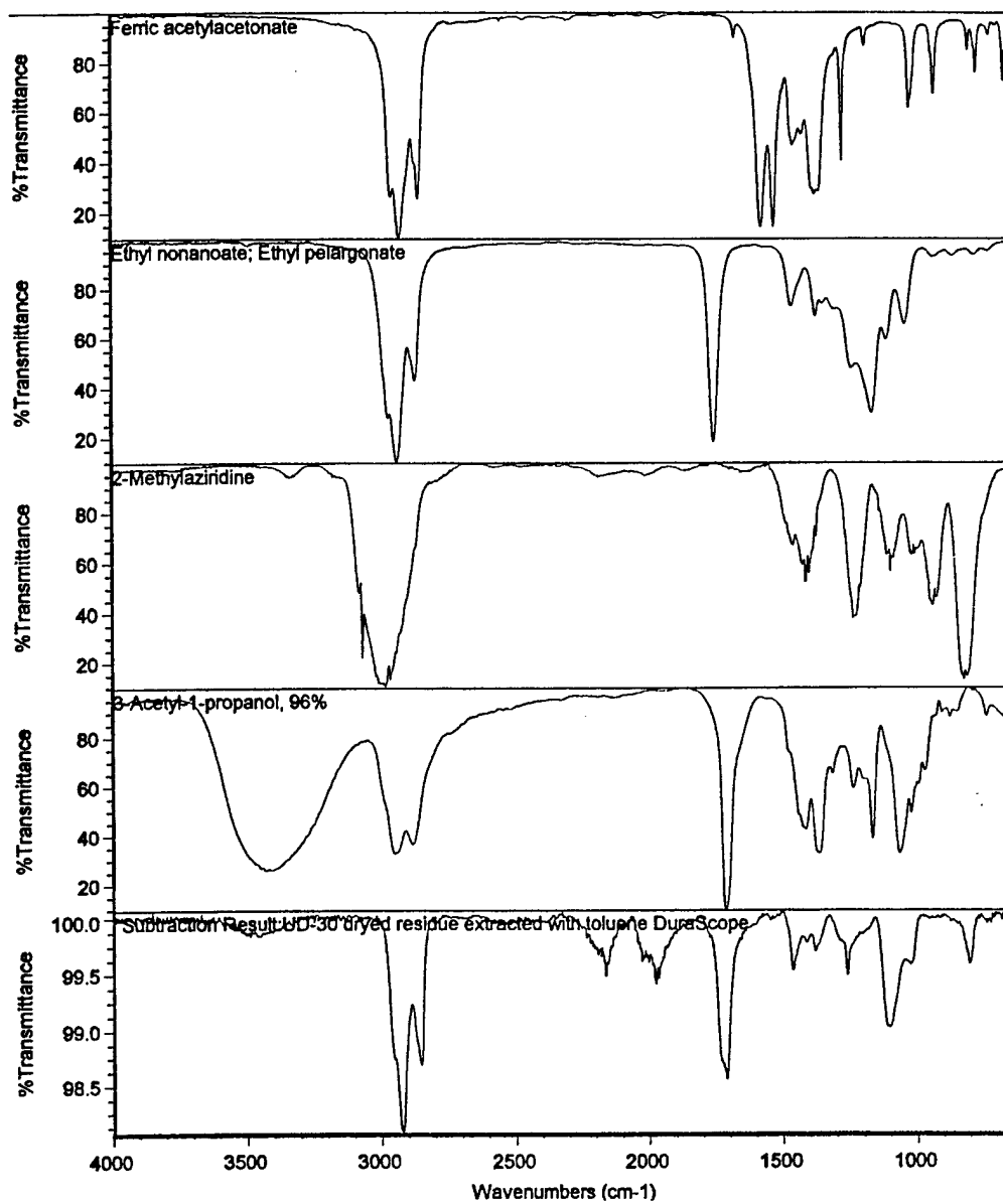
Figure A10. FTIR spectra of FeAA, ethyl pelargonate, methyl aziridine, 3-acetyl-1-propanol, and the residue from the toluene extracted aqueous dried residue from PU propellant.
