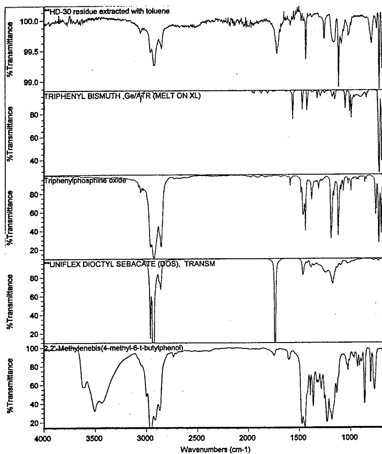
Figure A2. FTIR spectra of TPB, TPO, DOS, AO 2246, and the toluene extract from the dried residue of the aqueous extract from HTPB propellant.
