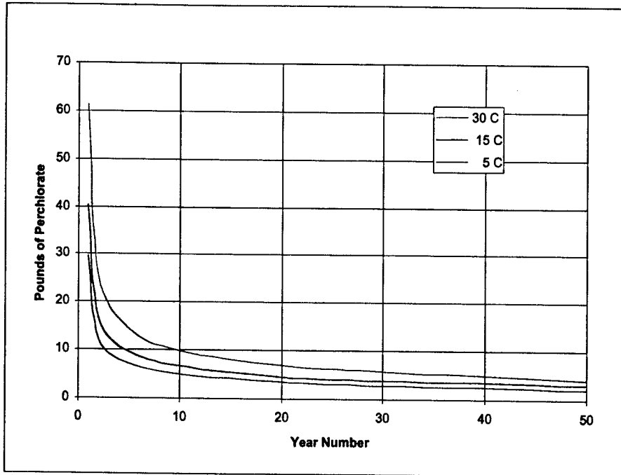
Figure 3.12. Effect of water temperature on probable perchlorate release during a specific year, lake, 15-s destruct, 1805 lb of propellant entering water.
