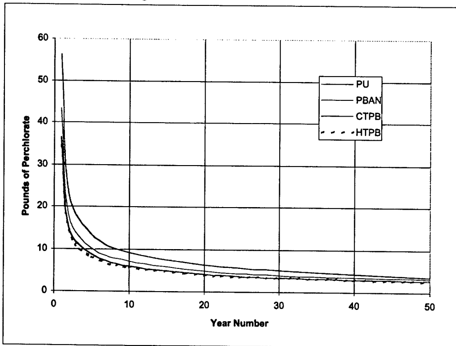
Figure 3.13. Various propellant types in lake. Probable perchlorate release during a specific year for 15-s destruct, 1805 lb of propellant entering water.
