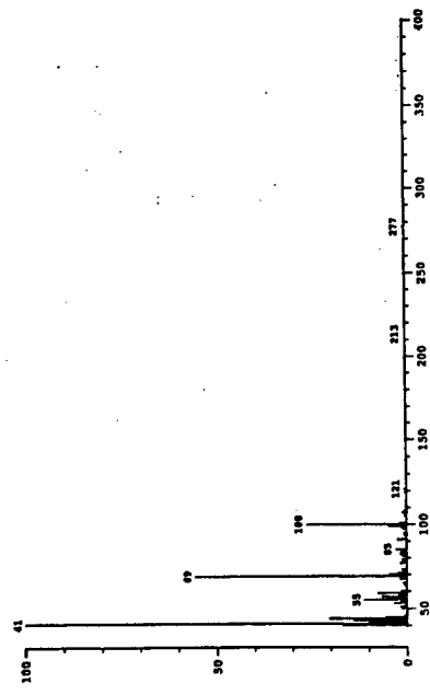
Figure A8 (continued). Mass Spectra of scan 200 and standard methyl methacrylate from SDBS library.
