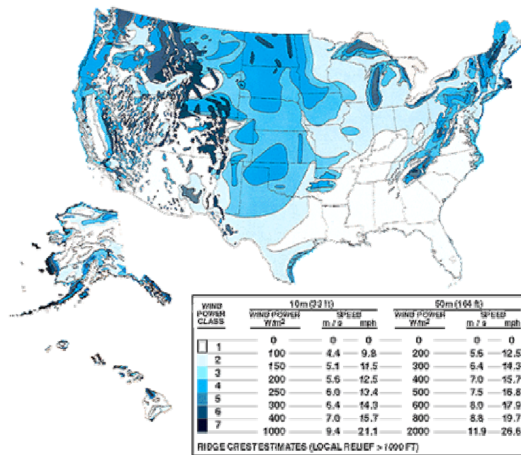
Figure 8. Wind Resource Map
