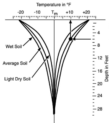
Figure 17. Soil Temperature Variations by Depth (DOE, 1995)
