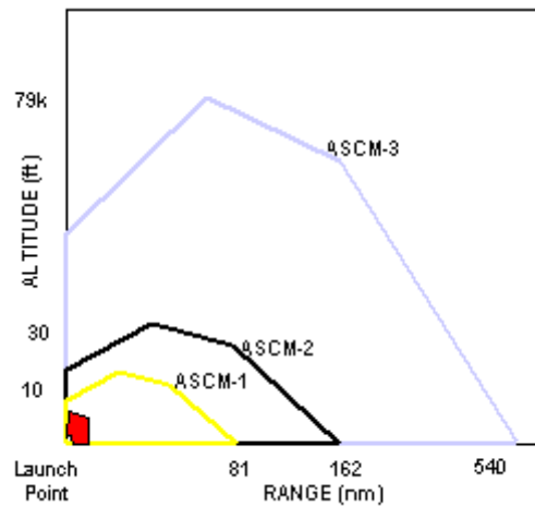
Figure 101. ASCM Threat Representative Flight Profiles
