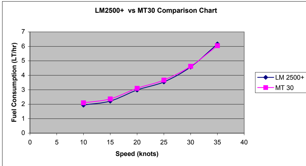
Figure 36. LM 2500+ and MT30 Fuel Consumption Comparison
