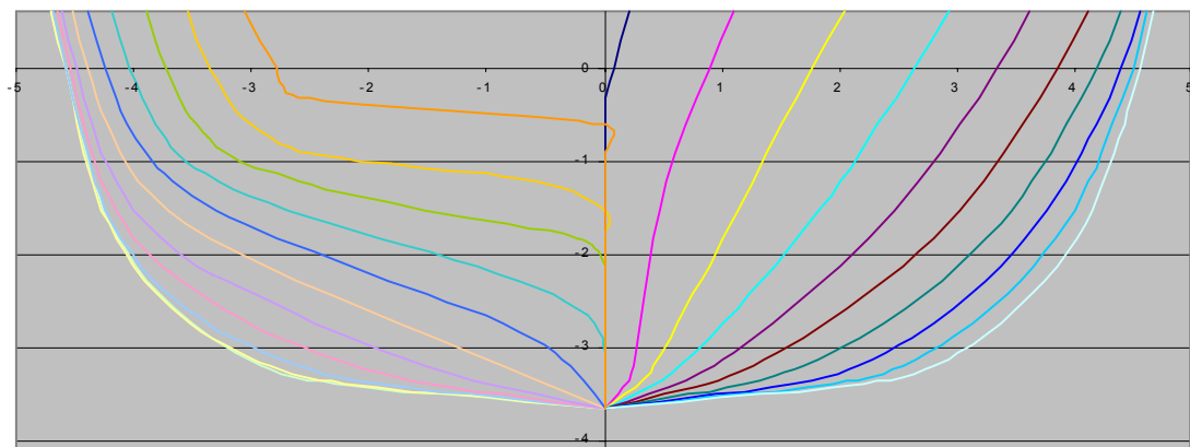
Figure 17. Body Plan of the Main Hull
