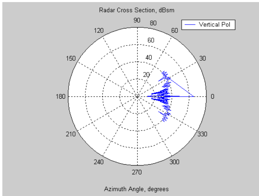
Figure 92. 10 GHz Radar Cross-Section Vertical Polarization
