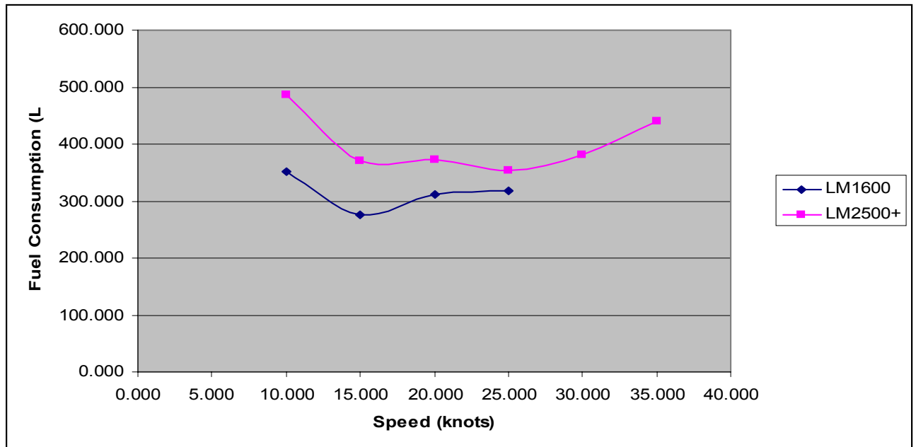
Figure 41. LM 1600 vs LM2500+ Fuel Consumptions
