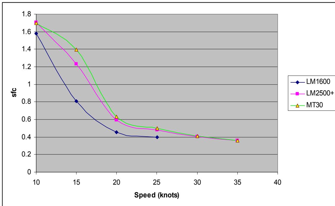
Figure 40. Specific Fuel Consumptions of Gas Turbines
