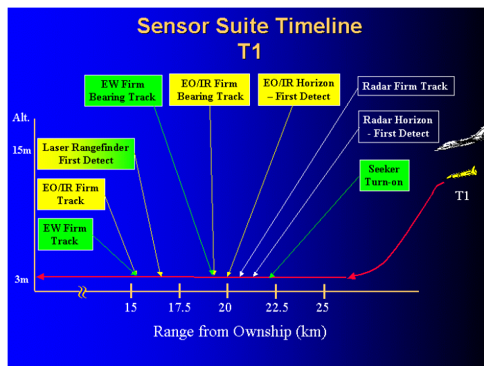
Figure 102. Sensors Suite Timeline for Threat 1
