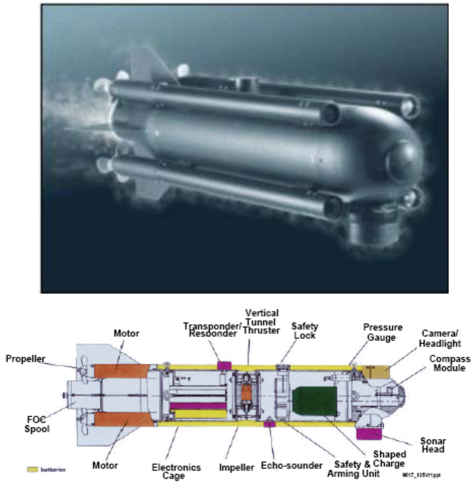
Figure 59. The AMNS Neutralizer
