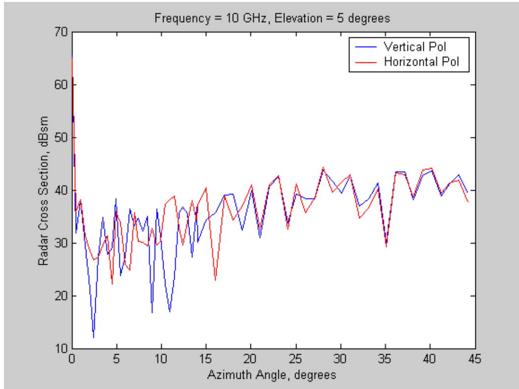
Figure 91. 10 GHz Radar Cross-Section Vertical and Horizontal Polarizations
