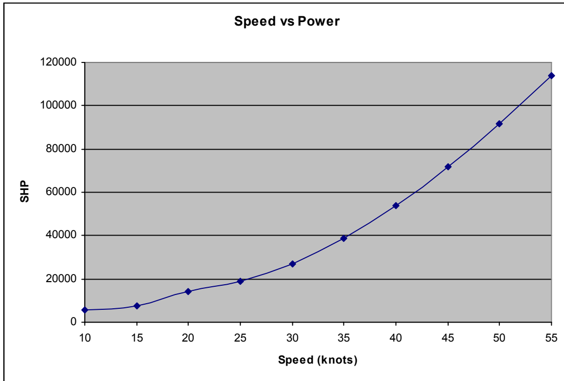
Figure 39. Speed vs Required Power
