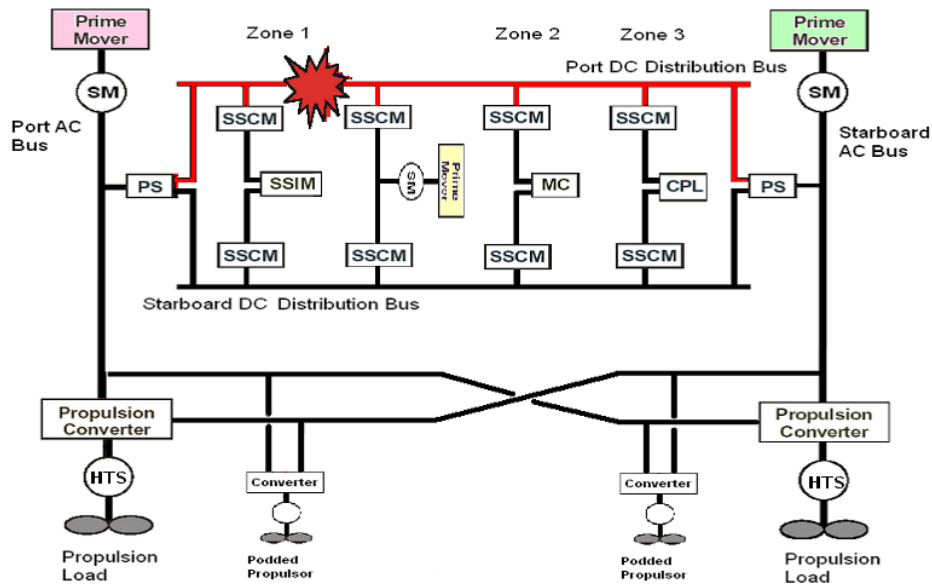
Figure 98. DC Bus Casualty Operation
