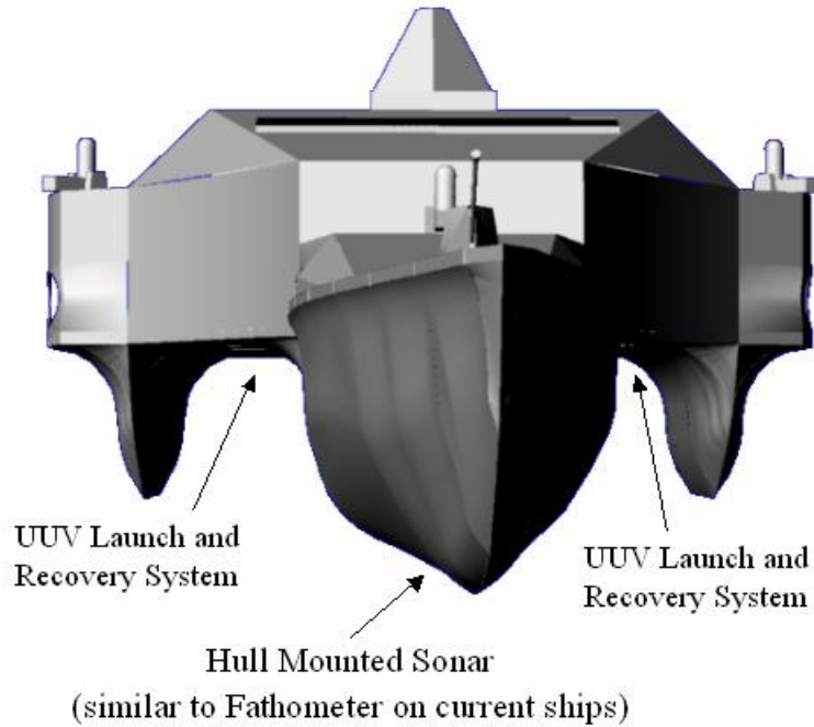
Figure 26. Bow Aspect of SEA SWAT Combat Systems
