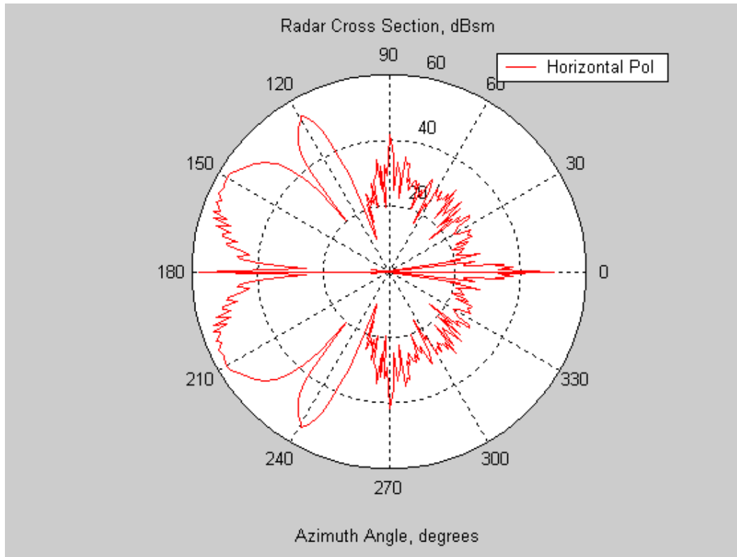
Figure 90. 1 GHz Radar Cross-Section Vertical Polarization
