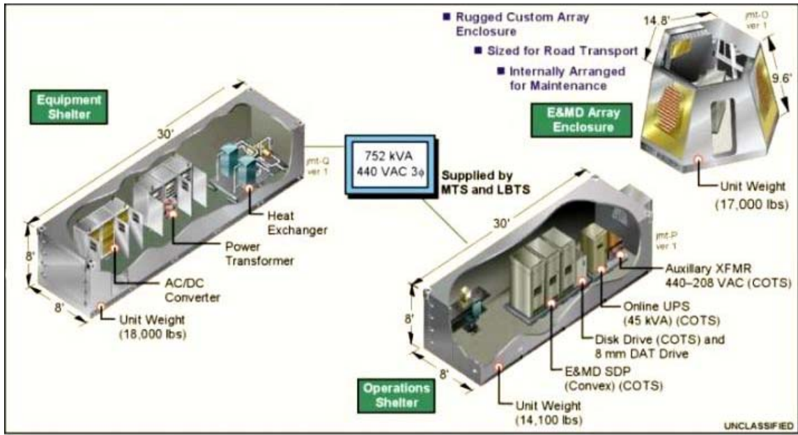
Figure 53. Estimated Size and Weight for MFR based on SPY 3
