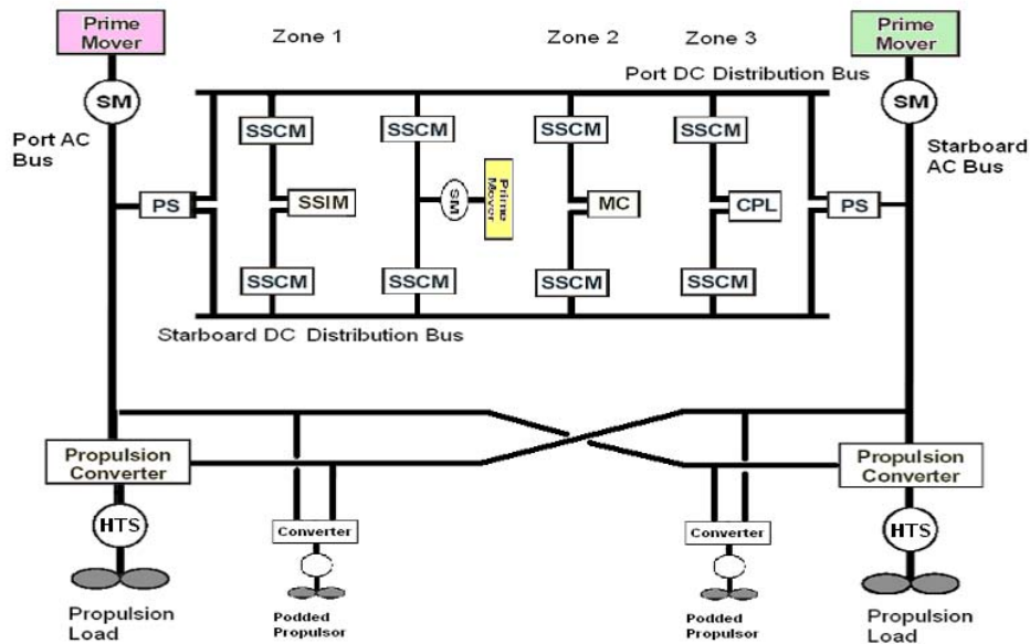
Figure 37. SEA SWAT ELECTRICAL DISTRIBUTION
