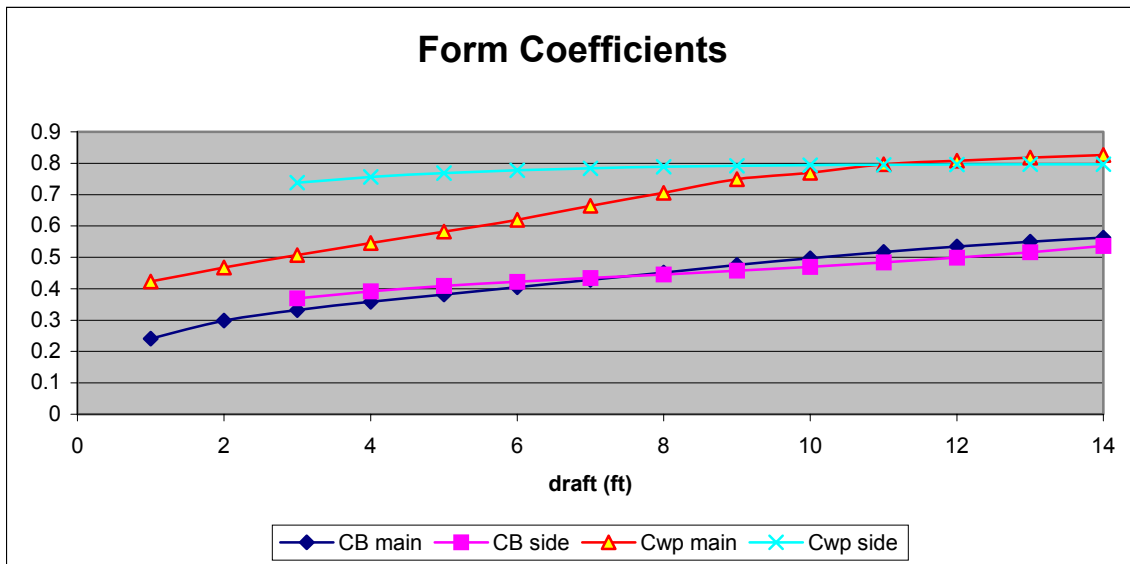
Figure 52. SEA SWAT Form Coefficients
