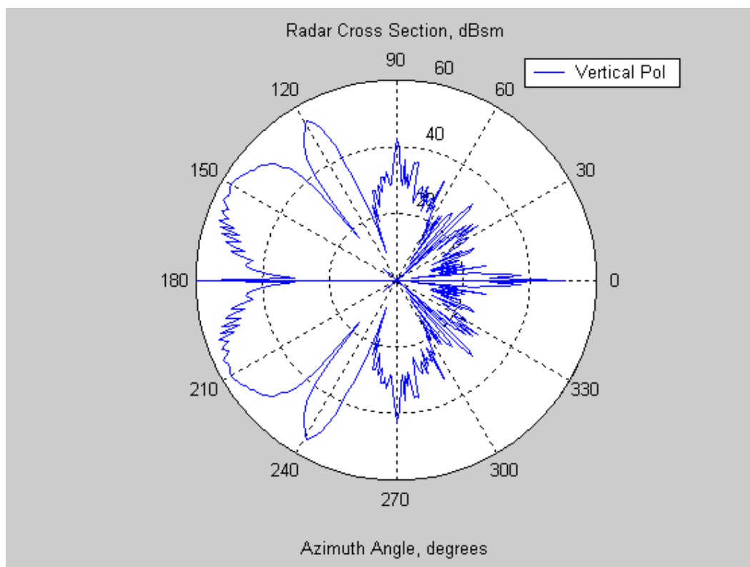
Figure 89. 1 GHz Radar Cross-Section Vertical Polarization
