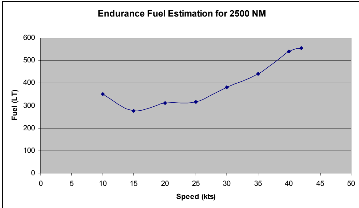
Figure 42. Endurance Fuel Estimation for 2500 NM
