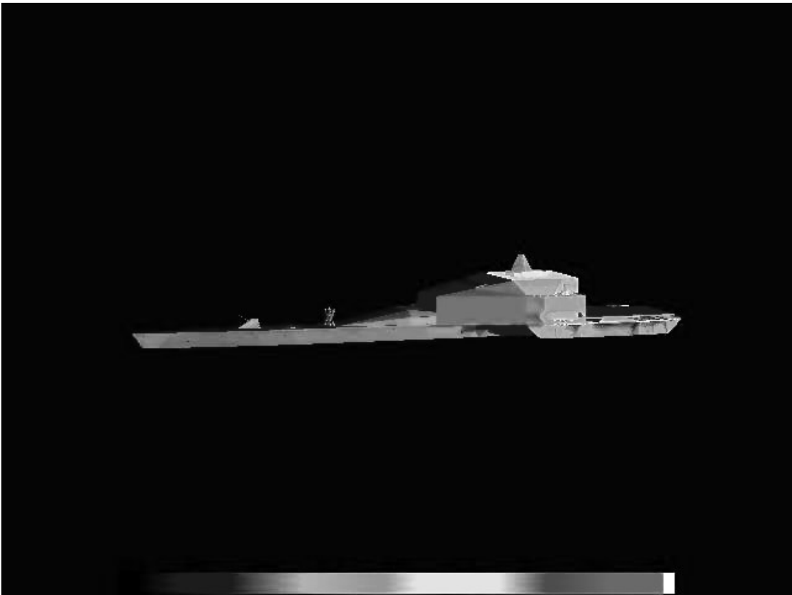
Figure 108. IR Signature Model Output
