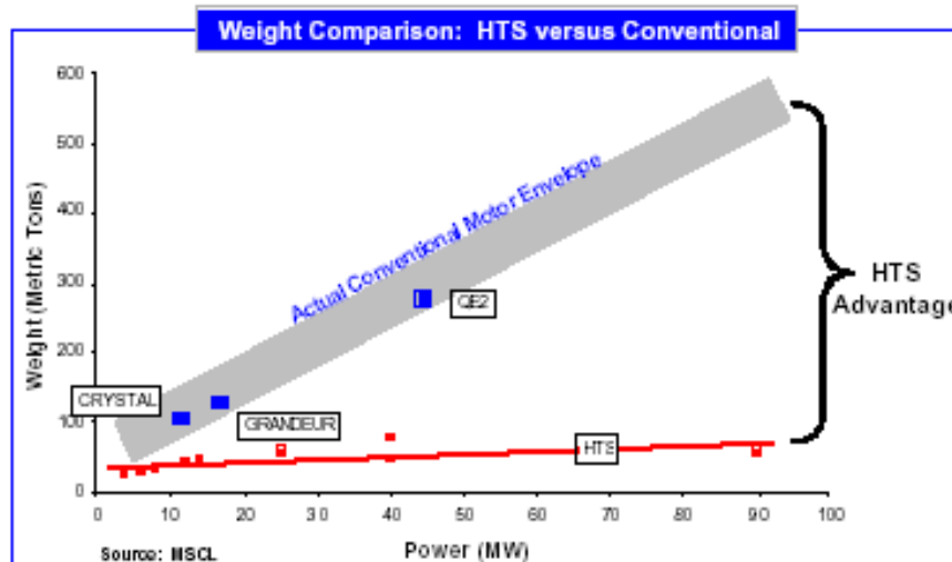
Figure 38. HTS vs. Conventional Weight Comparison
