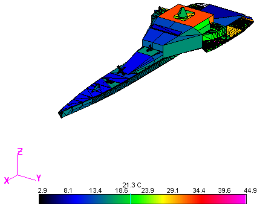
Figure 107. Temperature Model Simulation Output
