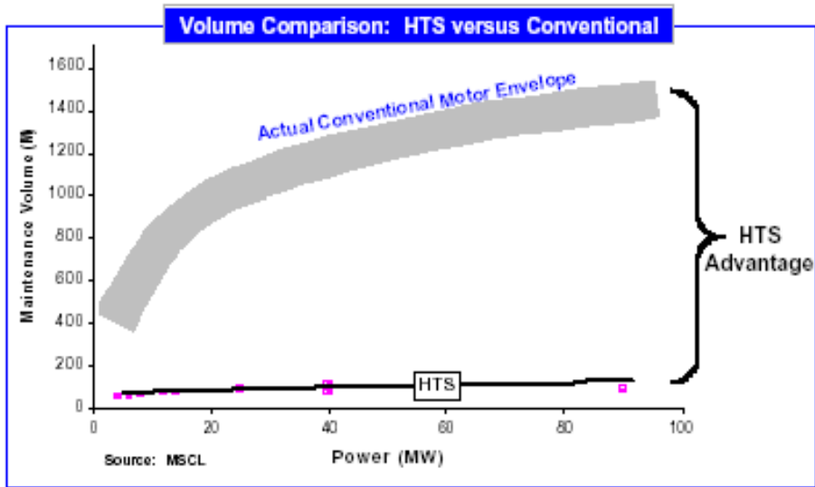
Figure 47. Volume Comparison HTS versus Conventional
