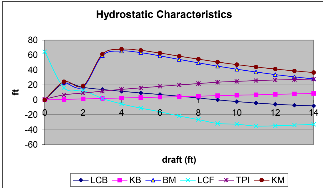
Figure 50. SEA SWAT Hydrostatic Characteristics
