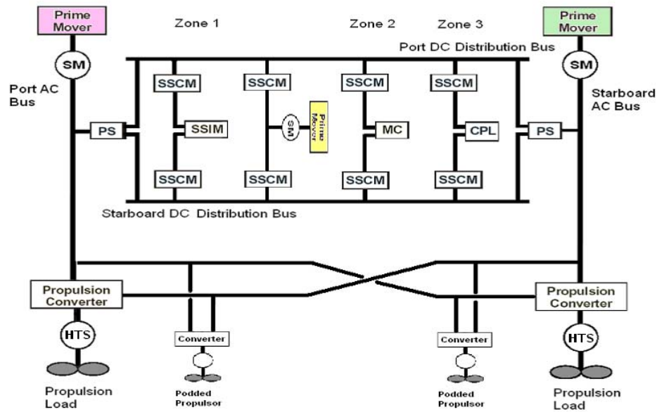
Figure 96. SEA SWAT Electrical Distribution
