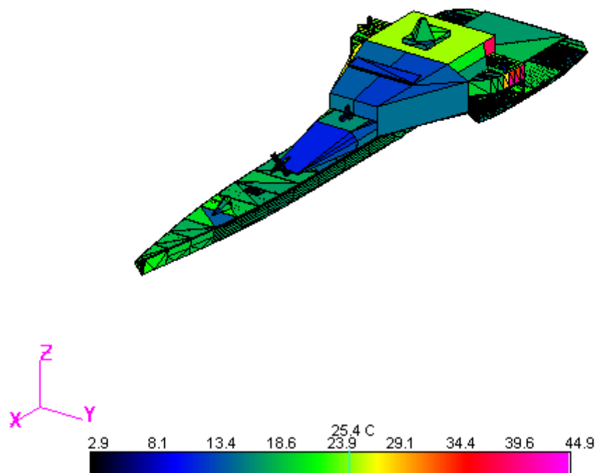
Figure 106. Temperature Model Simulation Output
