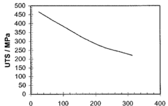
Tensile strength vs. temperature
