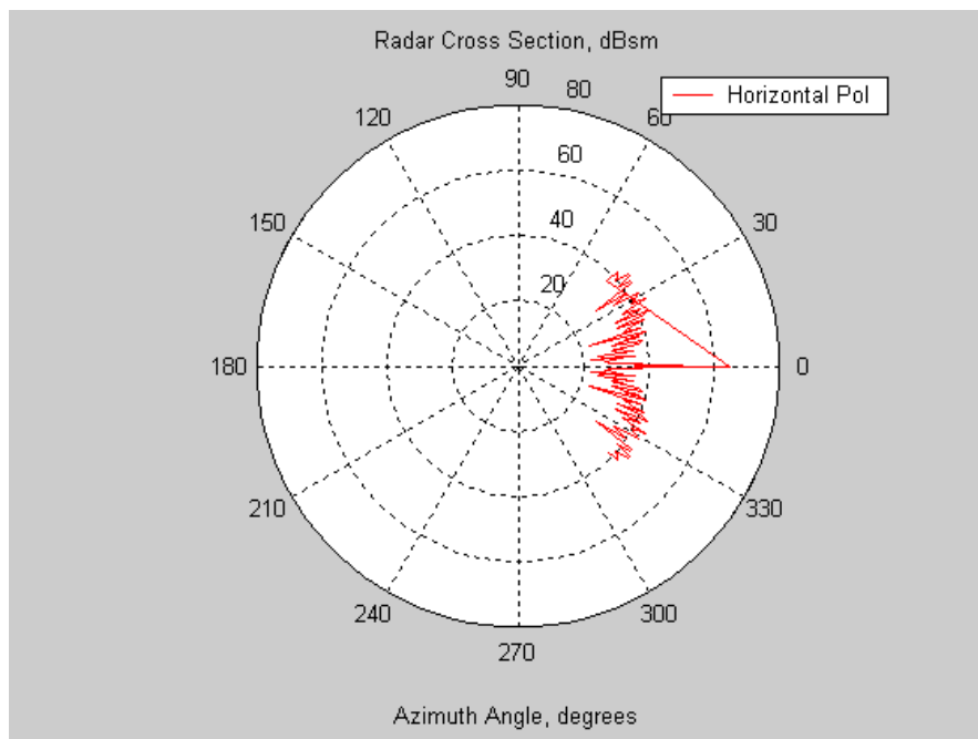
Figure 93. 10 GHz Radar Cross-Section Vertical Polarization
