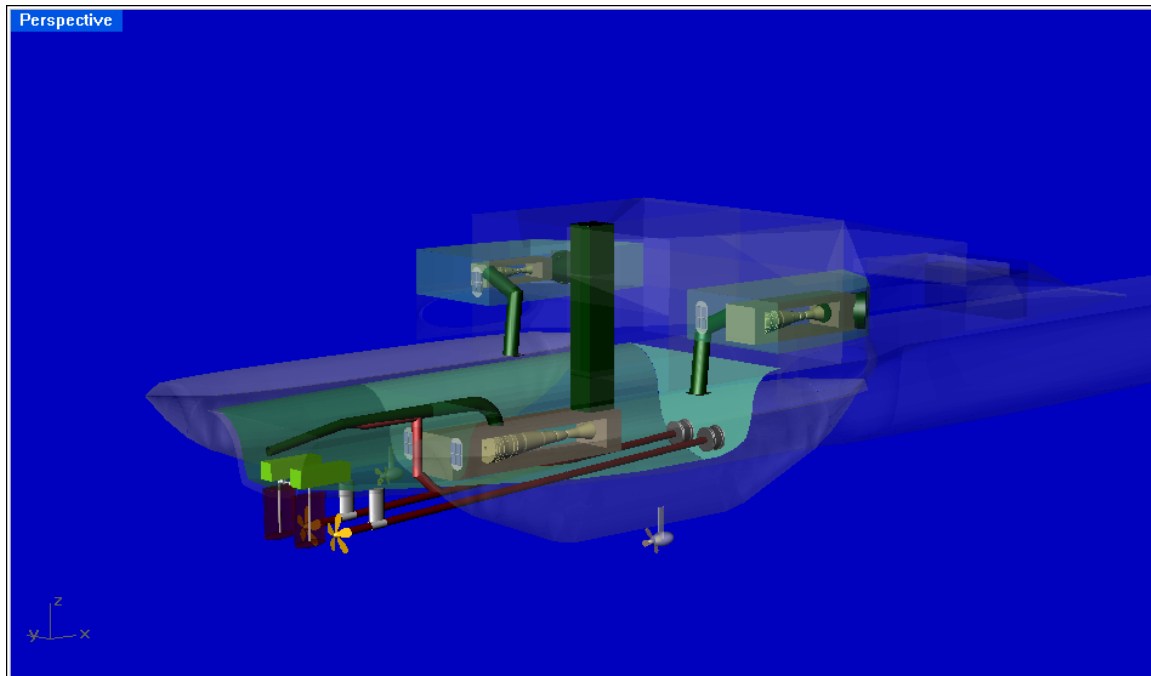
Figure 45. Gas Turbine Exhaust System
