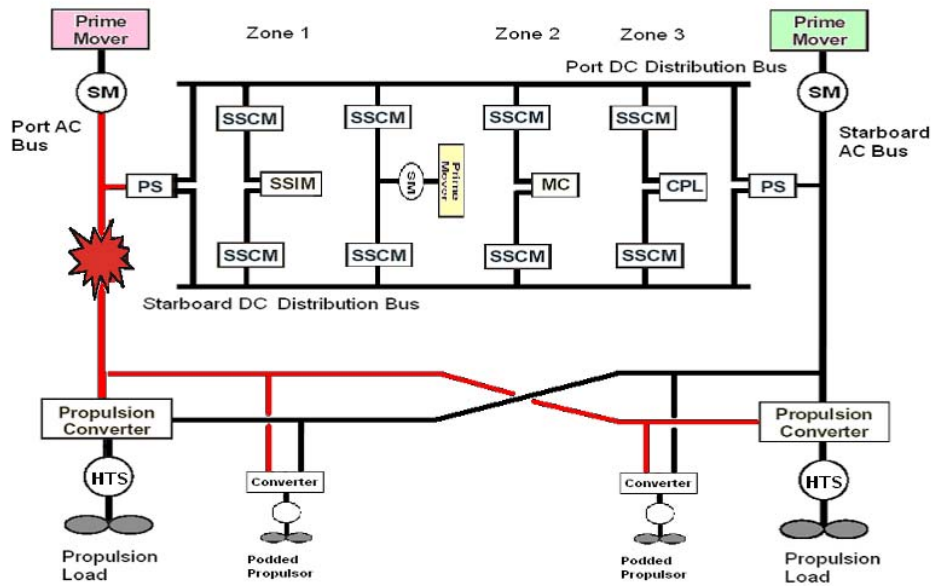
Figure 99. AC Bus Casualty Operation
