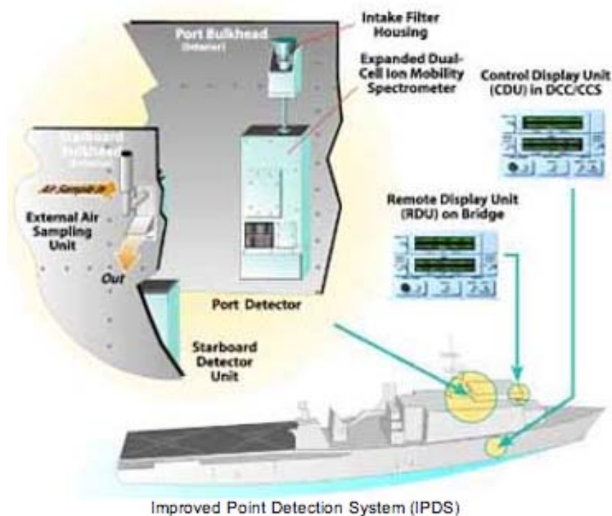
Figure 72. Improved Point Detection System
