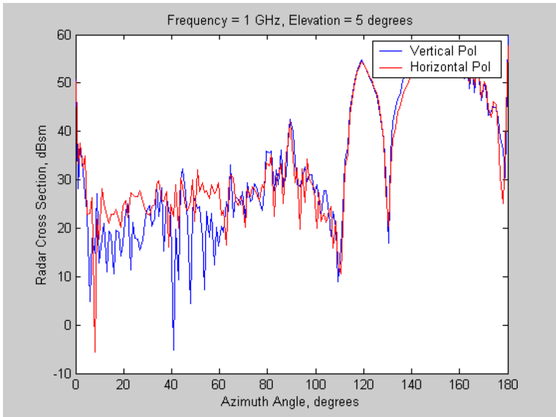
Figure 88. 1 GHz Radar Cross-Section in Vertical and Horizontal Polarizations
