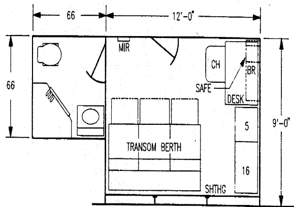
Figure 77. CO Sea Cabin and Bath
