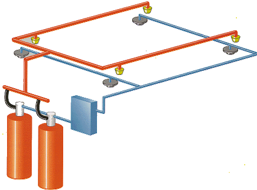
Figure 66. FM-200 (HFC-227) Fire Suppression System
