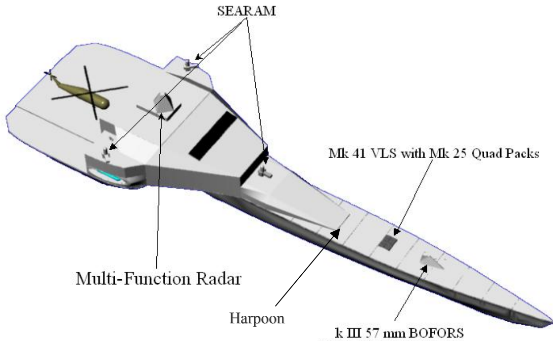
Figure 24. Topside SEA SWAT Combat Systems Layout
