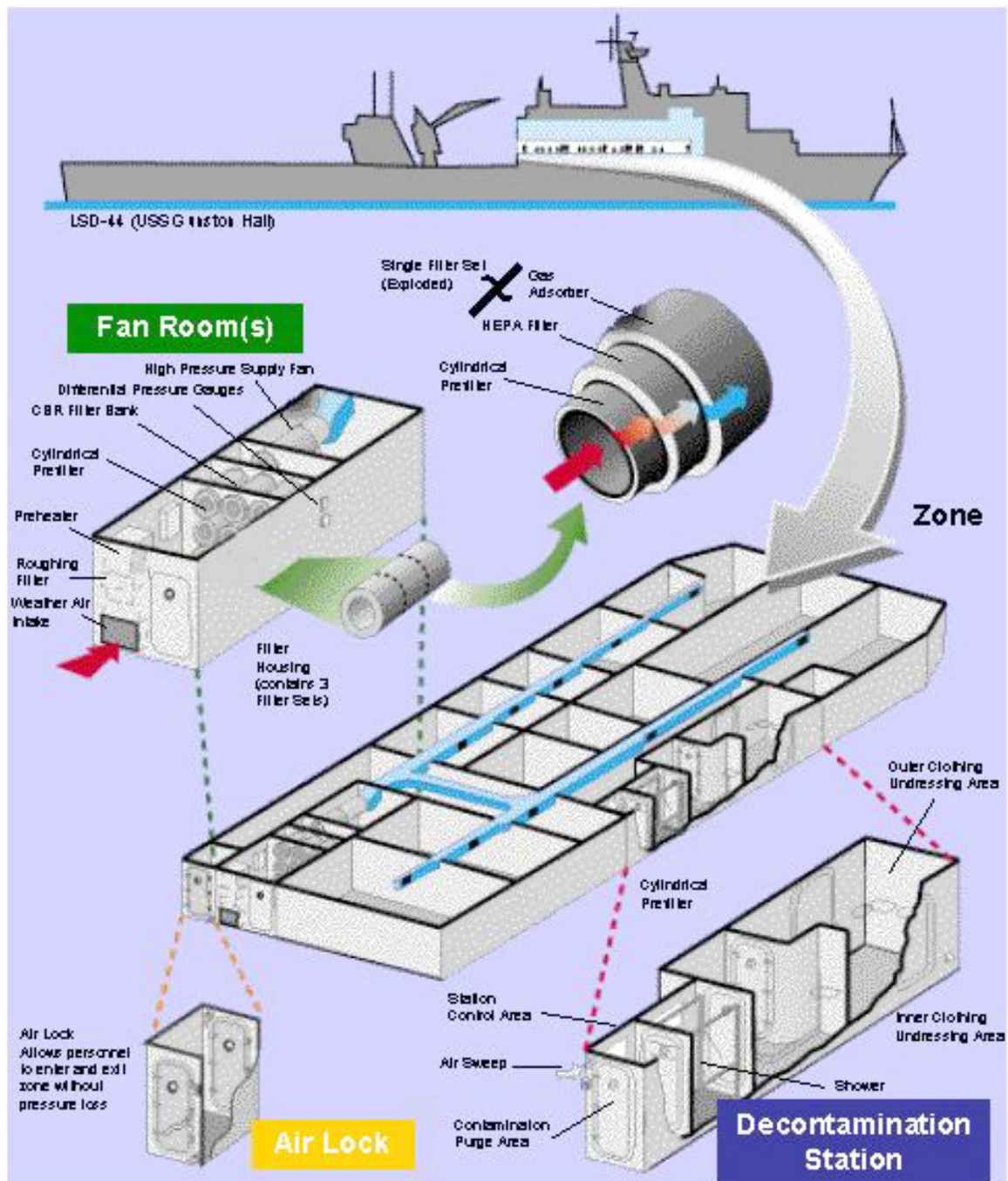
Figure 75. Typical Collective Protection System Installation
