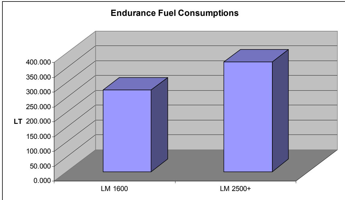
Figure 43. Endurance Fuel Consumption Comparison at 15 knots
