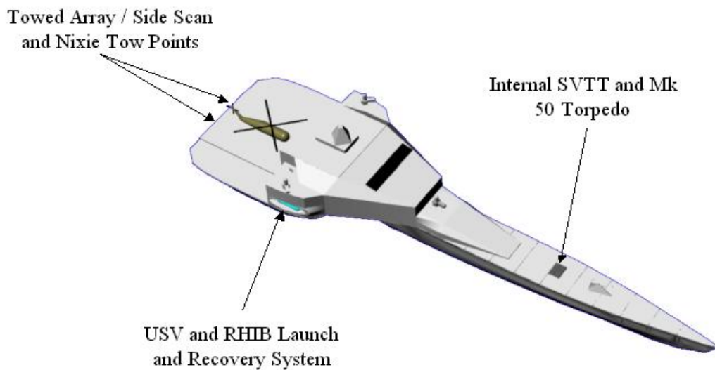
Figure 27. Top Down View of SEA SWAT
