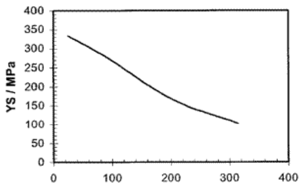
Yield strength vs. temperature
