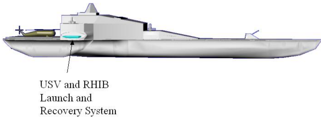
Figure 25. Profile of SEA SWAT
