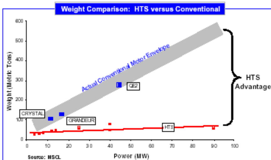
Figure 48. Weight Comparison HTS versus Conventional
