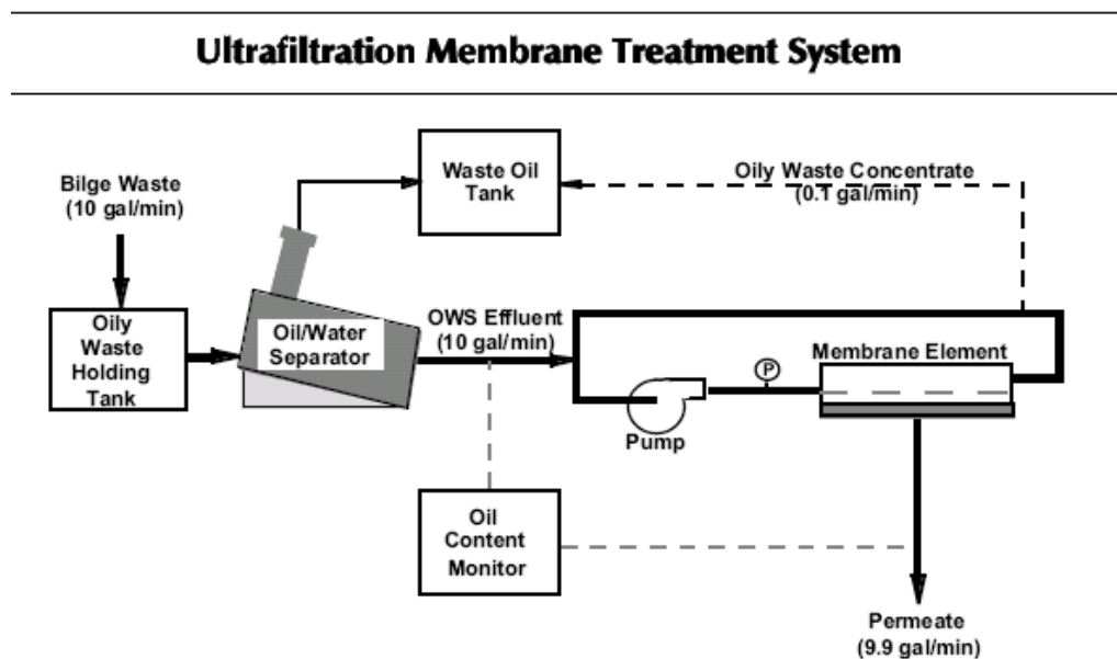
Figure 86. OWS System with Ultra-filtration Membrane
