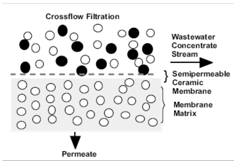
Figure 87. Ultra-filtration Membrane System
