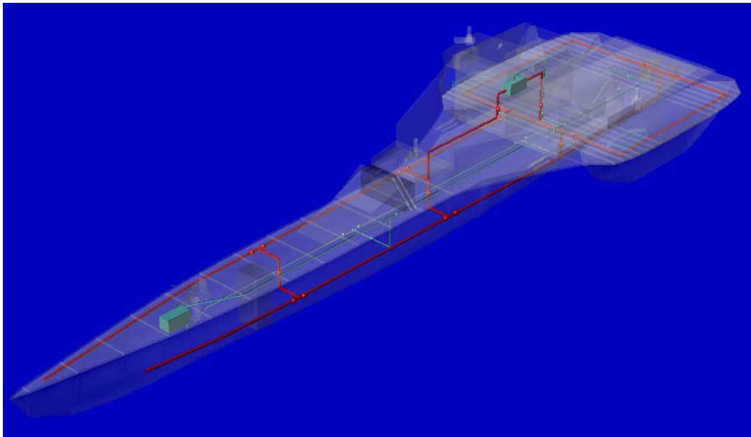
Figure 69. Firemain and AFFF System Notional Layout
