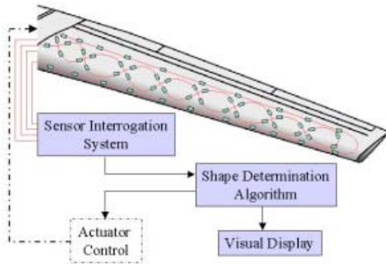
Figure 64. Force Base SPA Fiber Optic Embedded Wing Shape Sensing System
