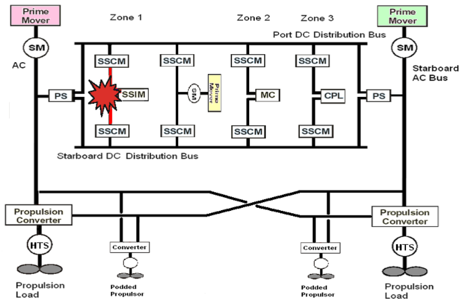
Figure 97. Intra-zone Casualty Operation
