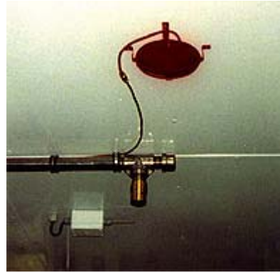
Figure 67. Flood System Storage Cylinder, Sensor and Nozzle
