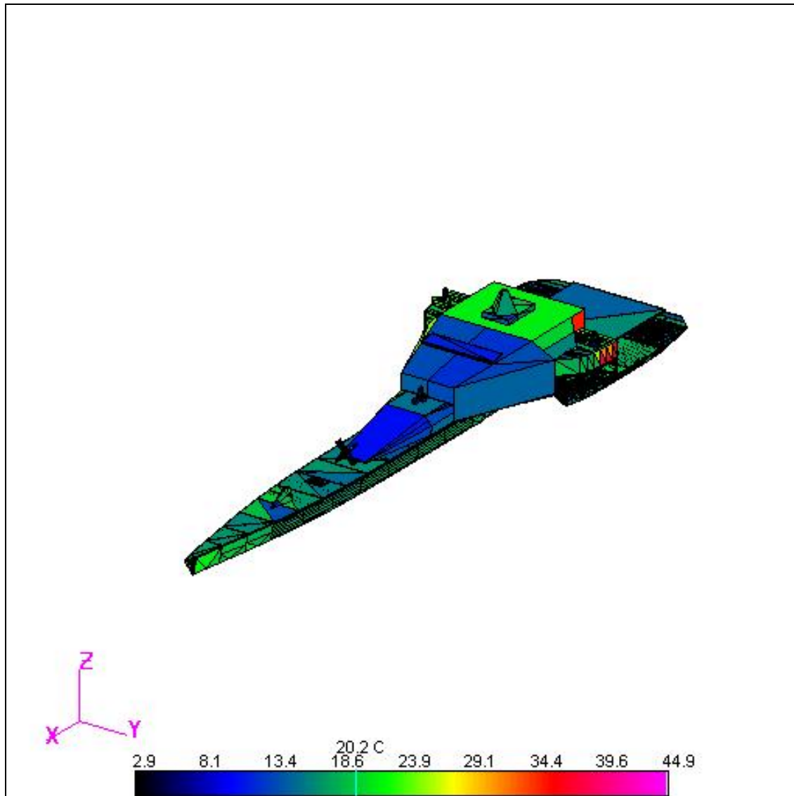
Figure 94. Temperature Model Simulation Output
