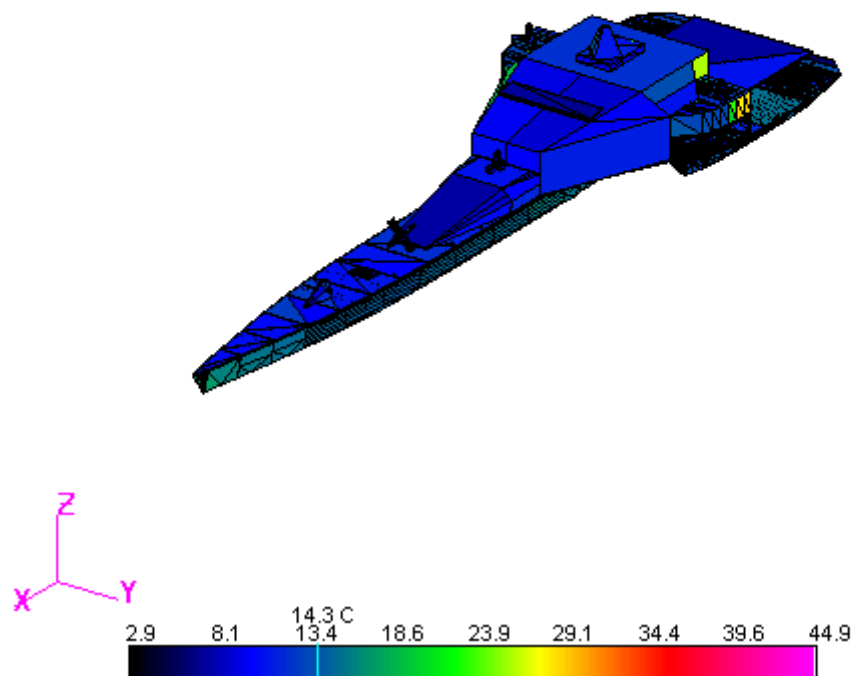
Figure 105. Temperature Model Simulation Output
