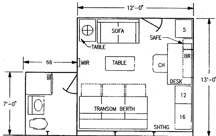
Figure 78. CO / XO Stateroom and Bath
