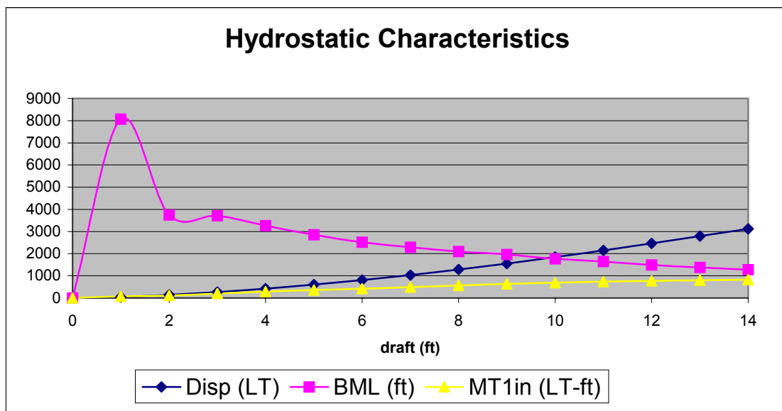
Figure 51. SEA SWAT Hydrostatic Characteristics
