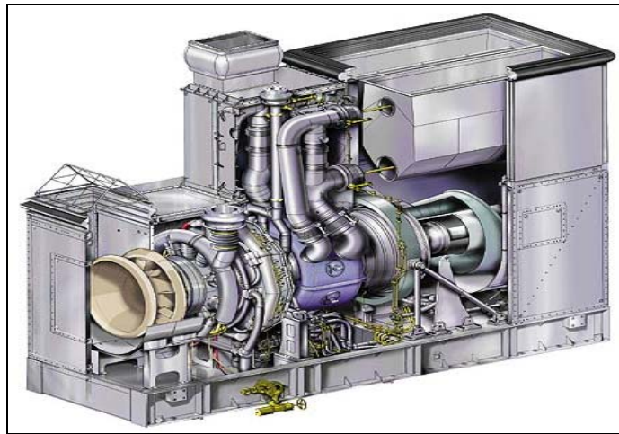
Figure 28. ICR WR21 Gas Turbine
