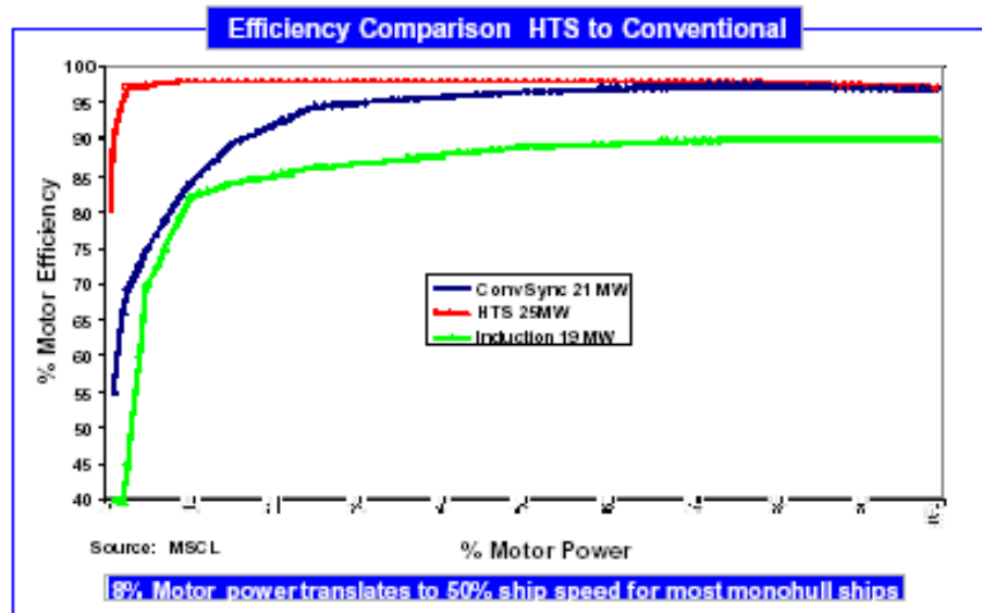
Figure 49. Efficiency Comparison HTS to Conventional
