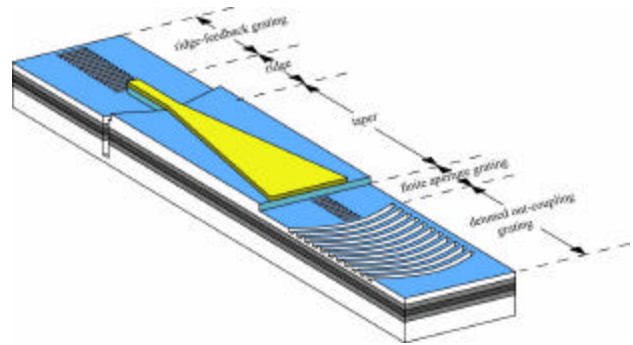
Figure 1 FATURL schematic
