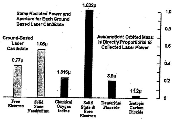
Figure 6. Wavelength Impact on Mass to LEO
