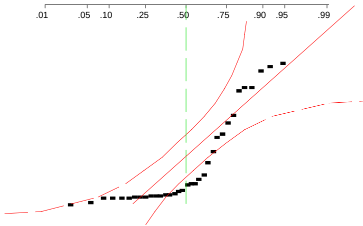
Figure 4. Normal Quantile Plot for Money Spent on all Projects
